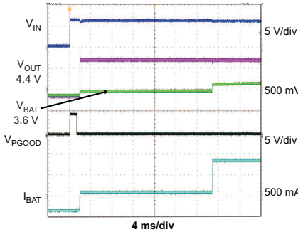
ADAPTER PLUG-IN BATTERY CONNECTED R_{LOAD} = 10\Omega
