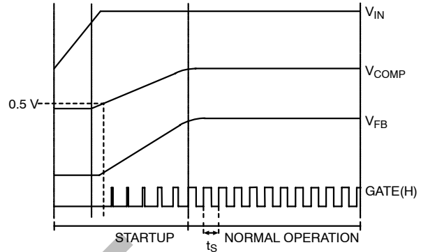
Figure 20. Idealized Waveforms
