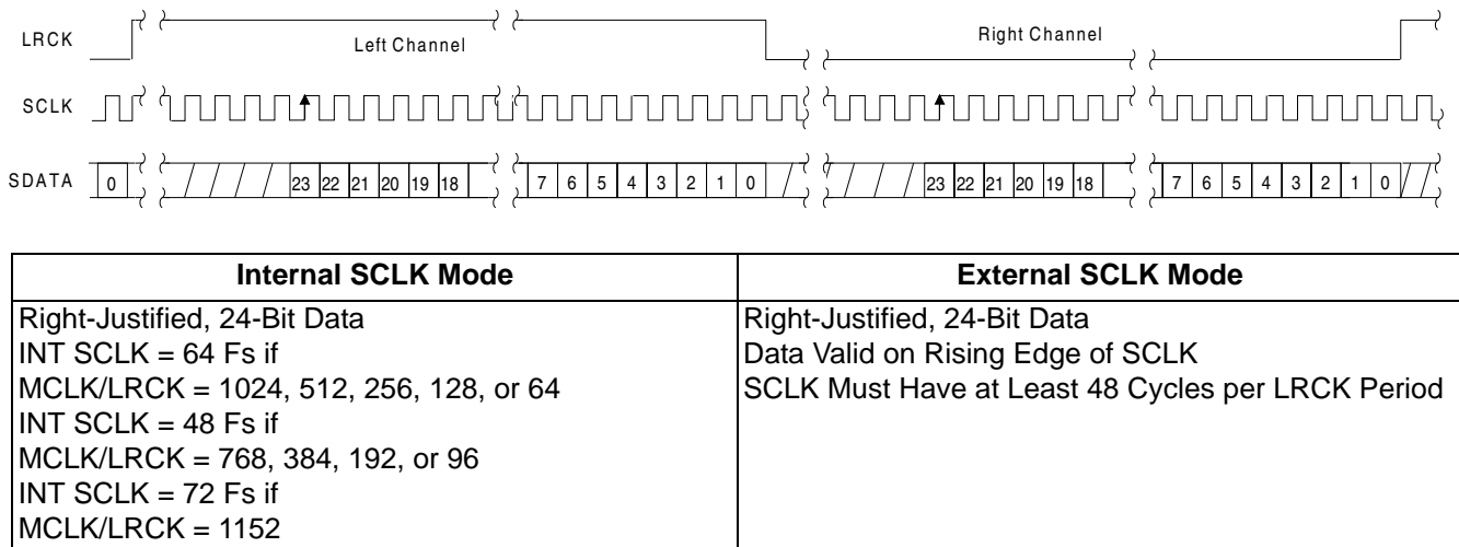
Figure 9. CS4361 Data Format (Right-Justified 24)
