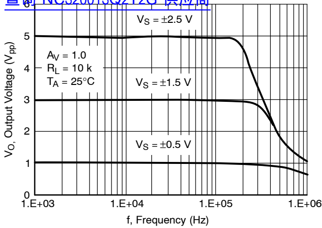
Figure 8. Output Voltage vs. Frequency
