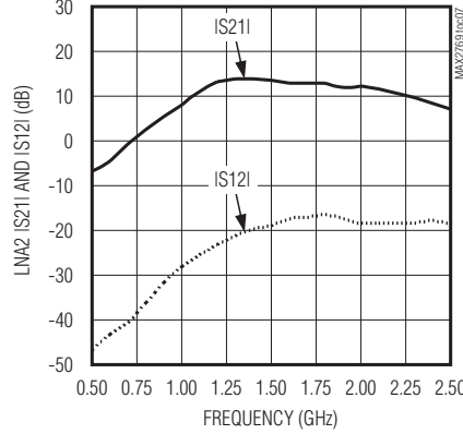
LNA2 IS211 AND IS121 vs. FREQUENCY
