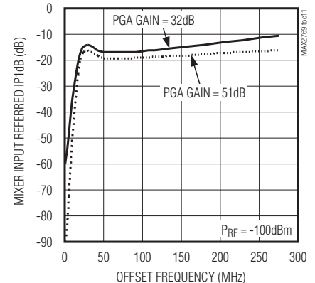
MIXER INPUT REFERRED IP1dB vs. OFFSET FREQUENCY
