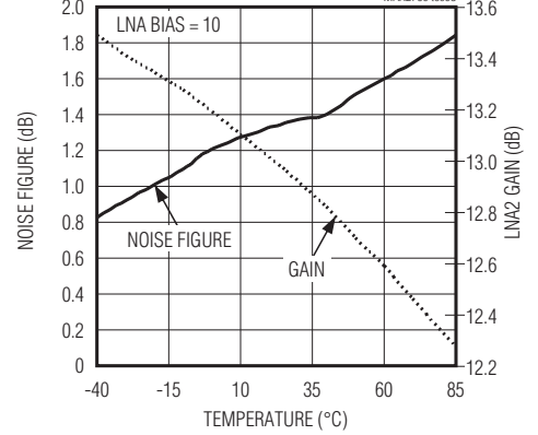
LNA2 GAIN AND NOISE FIGURE vs. TEMPERATURE
