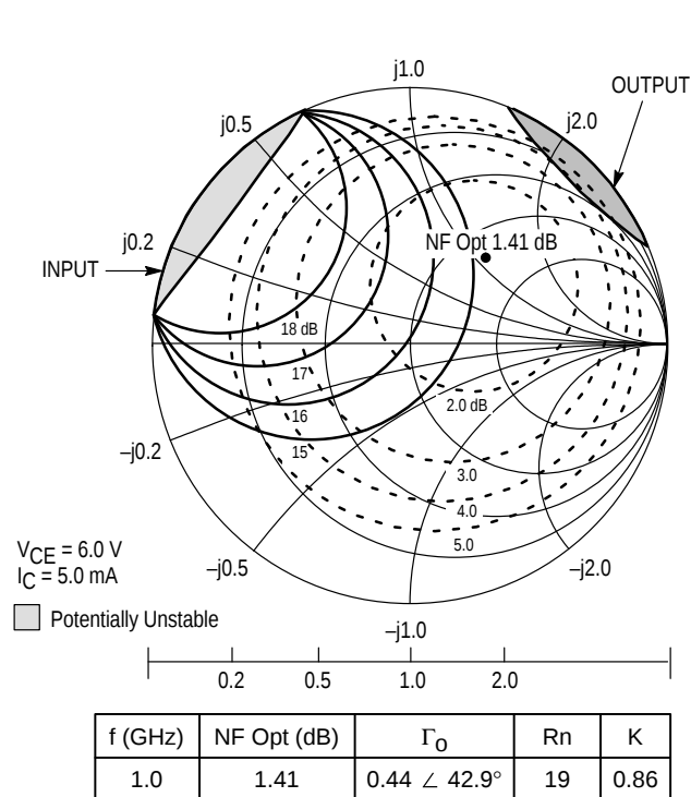
Figure 23. Constant Gain and Noise Figure Contours (f = 1.0 GHz)
