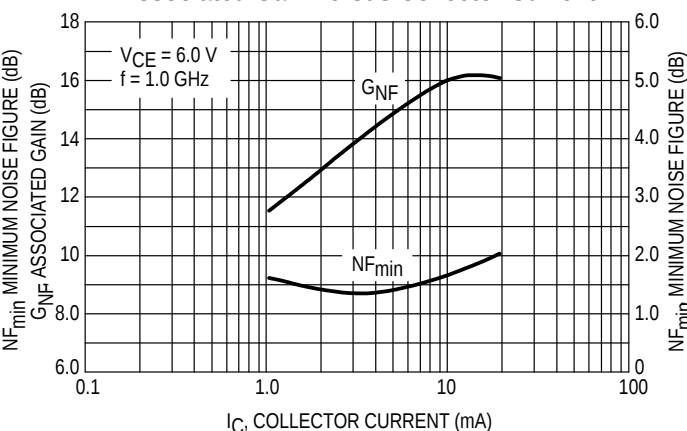
Figure 17. Minimum Noise Figure and Associated Gain versus Collector Current
