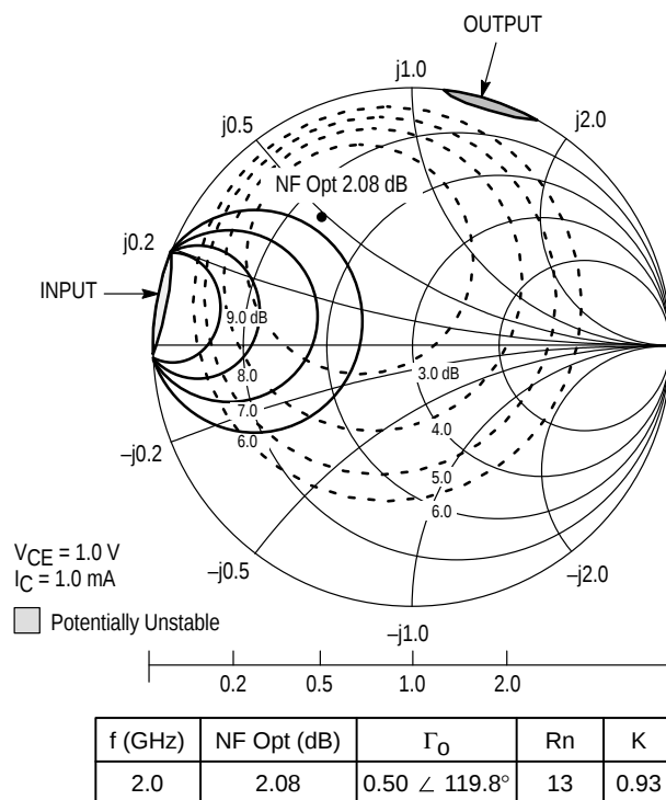
Figure 21. Constant Gain and Noise Figure Contours (f = 2.0 GHz)
