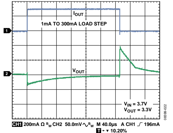
Figure 22. Load Transient Response, C_{OUT} = 1\mu F
