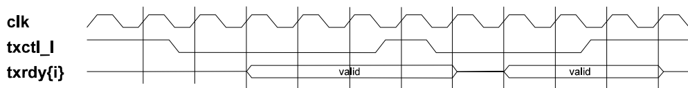
Figure 7-3. Transmit FIFO Control Timing
