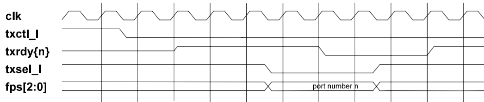
Figure 7-4. Transmit txrdy Timing
