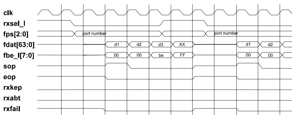
Figure 7-11. Receive Header Replay Timing
