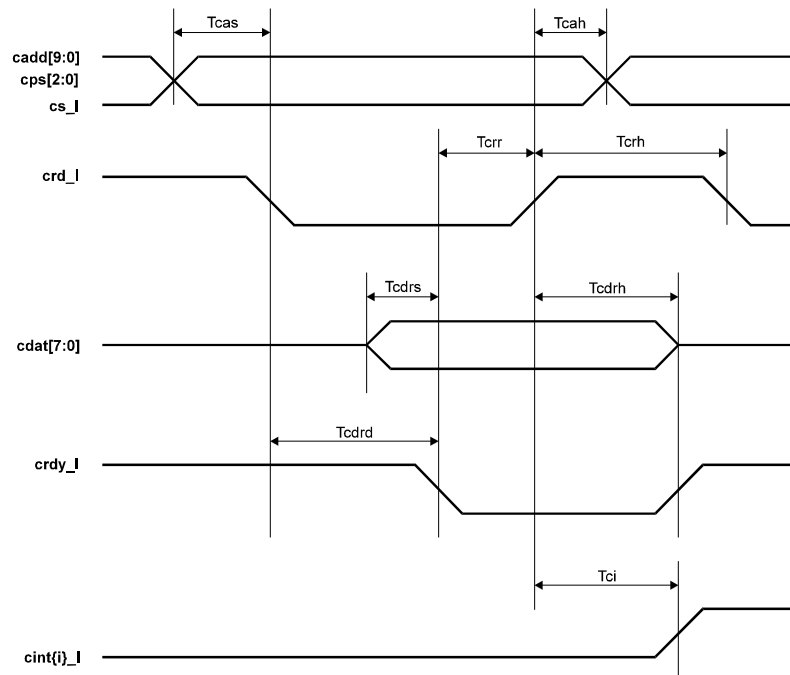
Figure 8-3. CPU Port Read Timing Diagram
