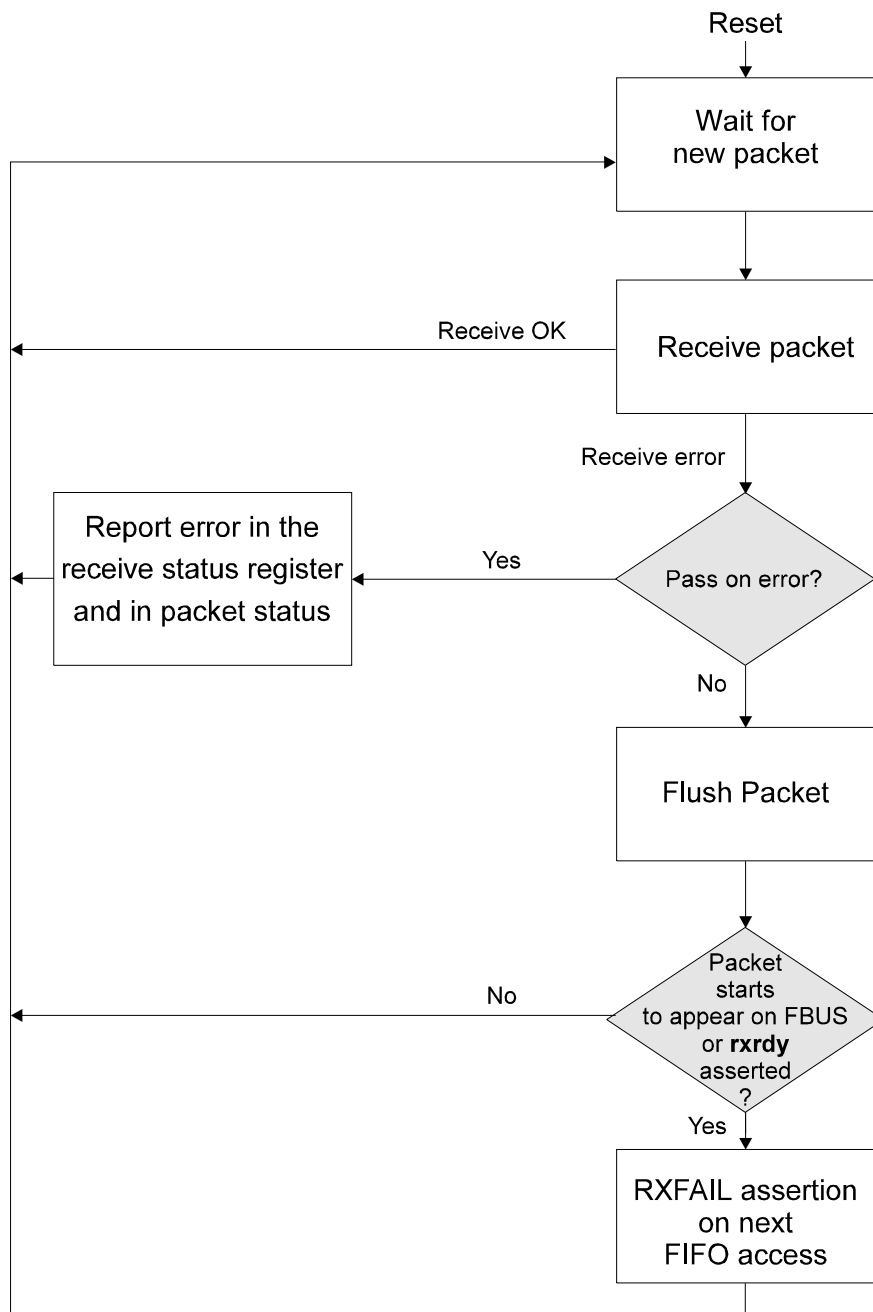
Figure 4-2. Receive Flow Diagram
