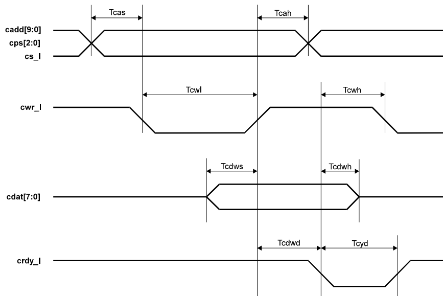
Figure 8-4. CPU Port Write Timing Diagram
