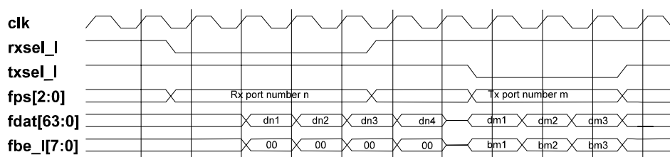
Figure 7-16. Consecutive Receive-Transmit Timing
