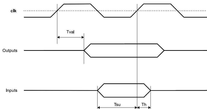
Figure 8-2. FIFO Bus Signals Timing Diagram
