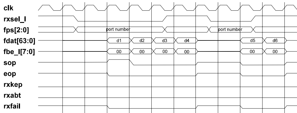
Figure 7-5. Receive Start-of-Packet Timing
