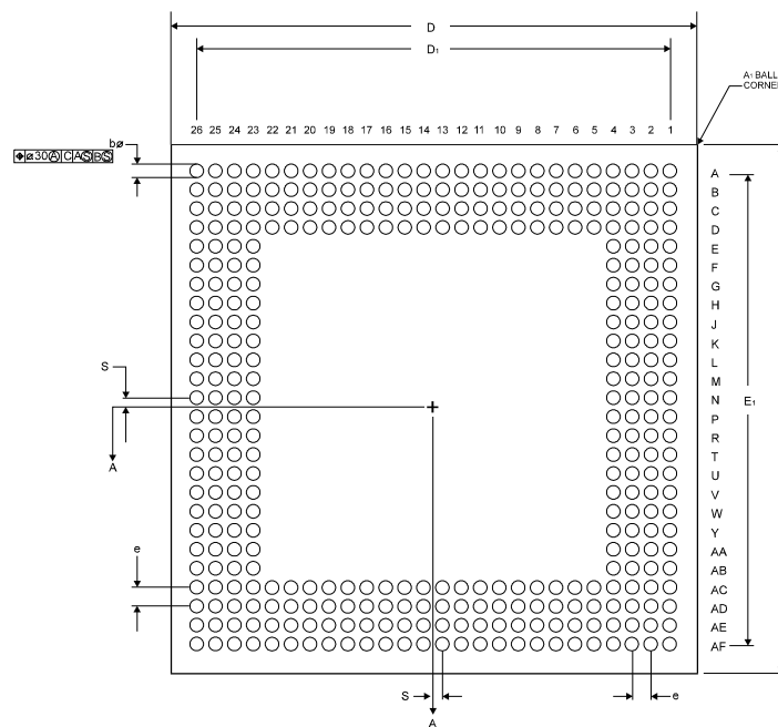
Figure 9-2. 352-BGA Package - Bottom View
