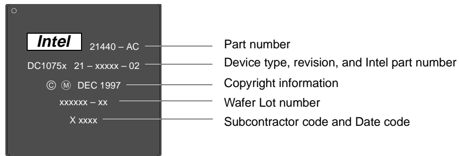
Figure 9-1. Part Marking
