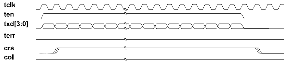
Figure 7-18. Packet Transmission Timing
