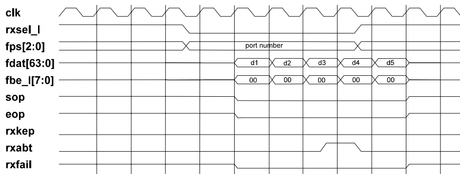
Figure 7-9. Receive rxabt Timing
