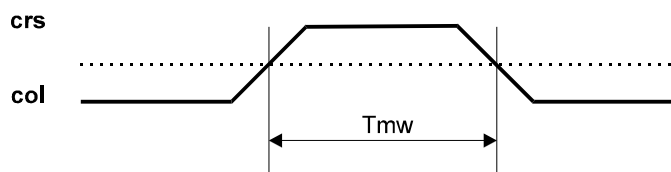
Figure 8-8. MII/SYM Port Carrier Sense and Collision Timing Diagram
