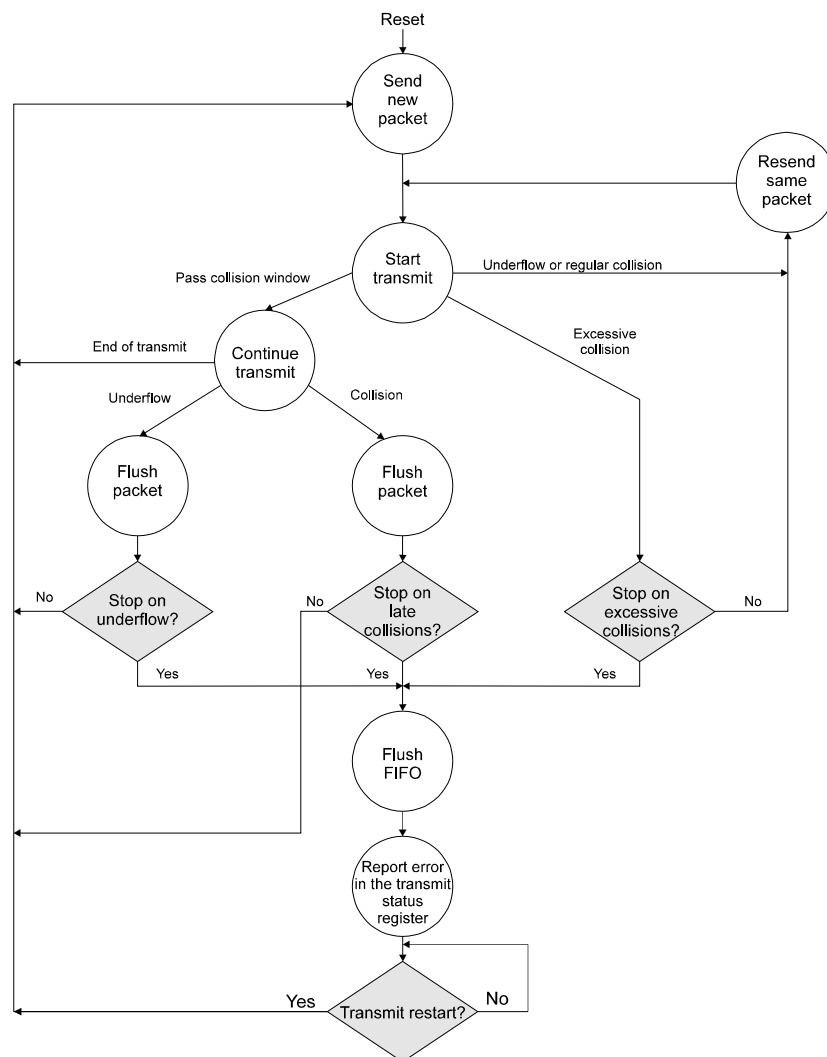
Figure 4-1. Transmit Flow Diagram
