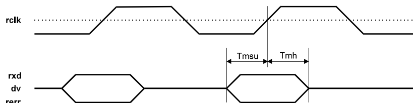
Figure 8-7. MII/SYM Port Receive Timing Diagram
