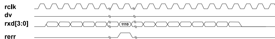
Figure 7-21. False Carrier Timing
