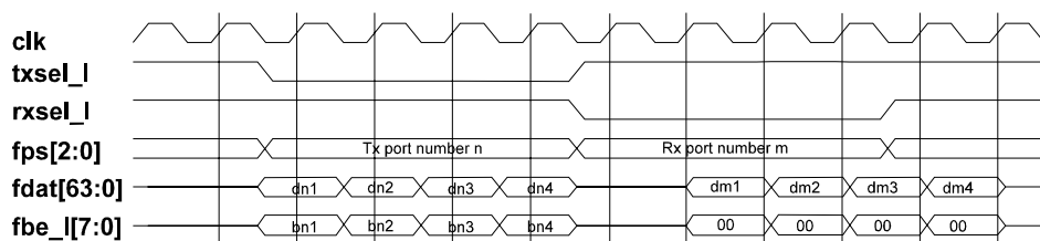
Figure 7-15. Consecutive Transmit-Receive Timing
