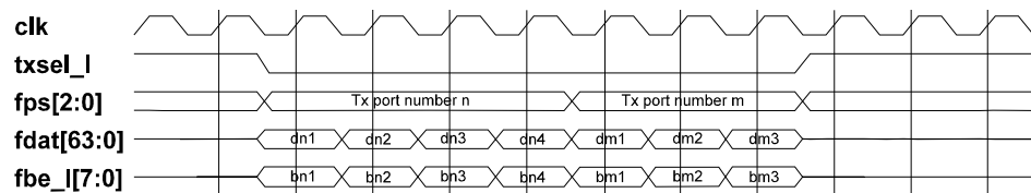
Figure 7-14. Consecutive Transmit-Transmit Timing
