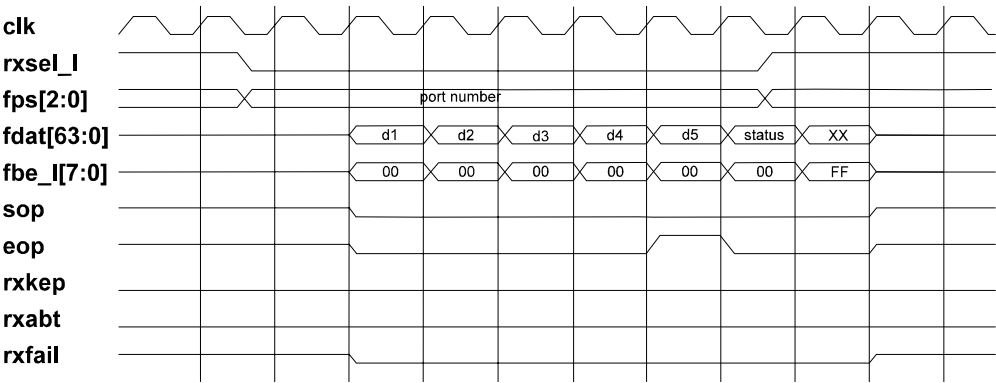
Figure 7-6. Receive End-of-Packet Timing
