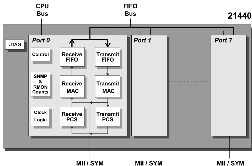
Figure 1-1. 21440 Controller Block Diagram
