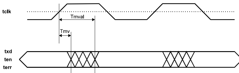
Figure 8-6. MII/SYM Port Transmit Timing Diagram
