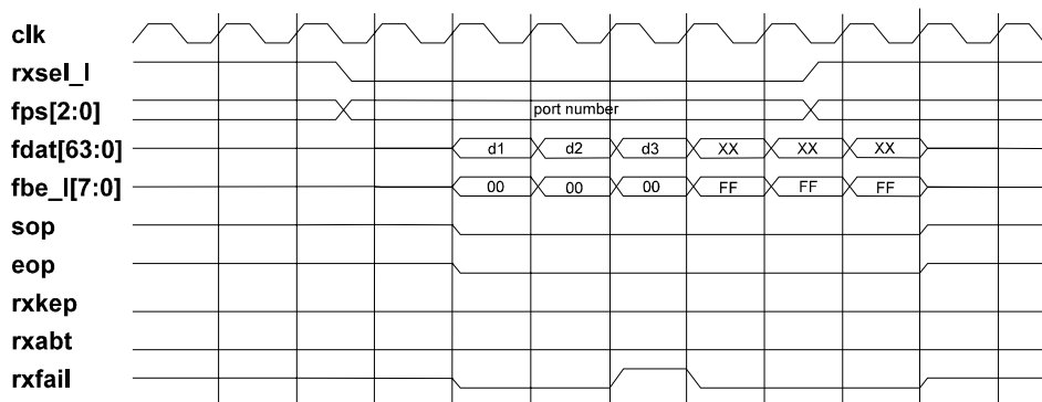
Figure 7-8. Receive rxfail Timing
