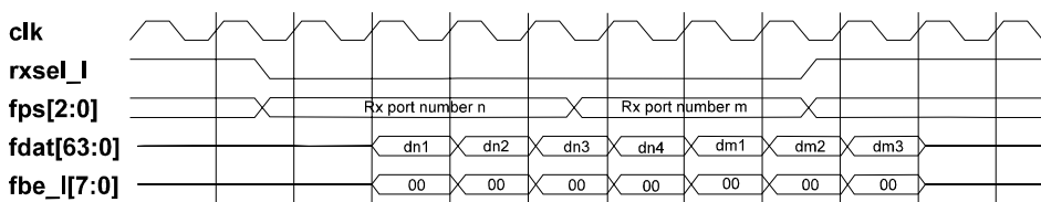
Figure 7-17. Consecutive Receive-Receive Timing
