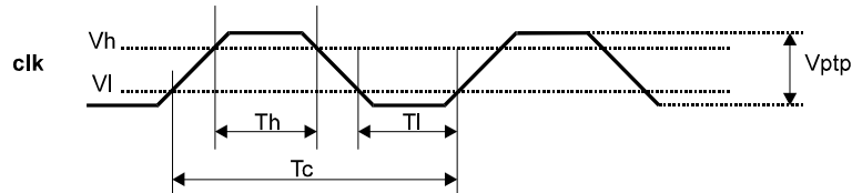
Figure 8-1. FIFO Bus Clock Timing Diagram
