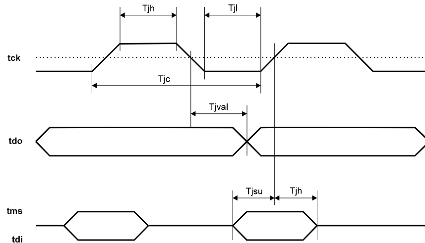
Figure 8-9. JTAG Port Timing Diagram
