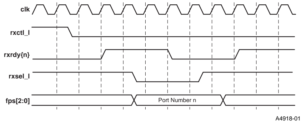
Figure 7-13. Receive rxrdy Timing
