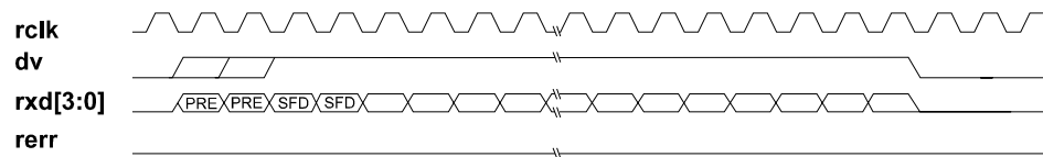
Figure 7-19. Packet Reception Timing
