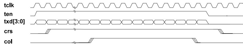
Figure 7-20. Transmission with Collision Timing
