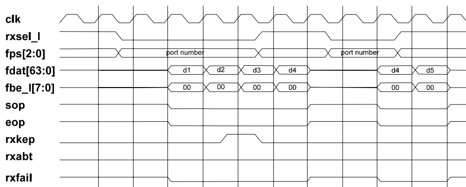
Figure 7-10. Receive rxkep Timing
