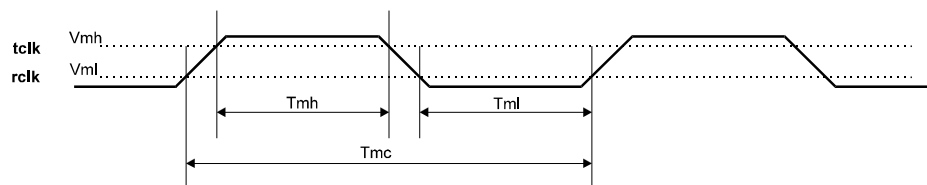
Figure 8-5. MII/SYM Clock Timing Diagram
