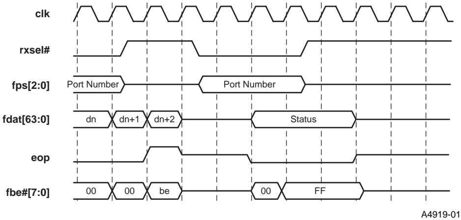
Figure 7-7. Fastest Receive Reaccess After EOP
