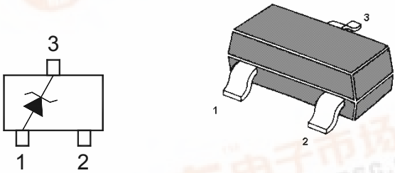
1. ANODE 3. CATHODE SOT-23 Plastic Package
