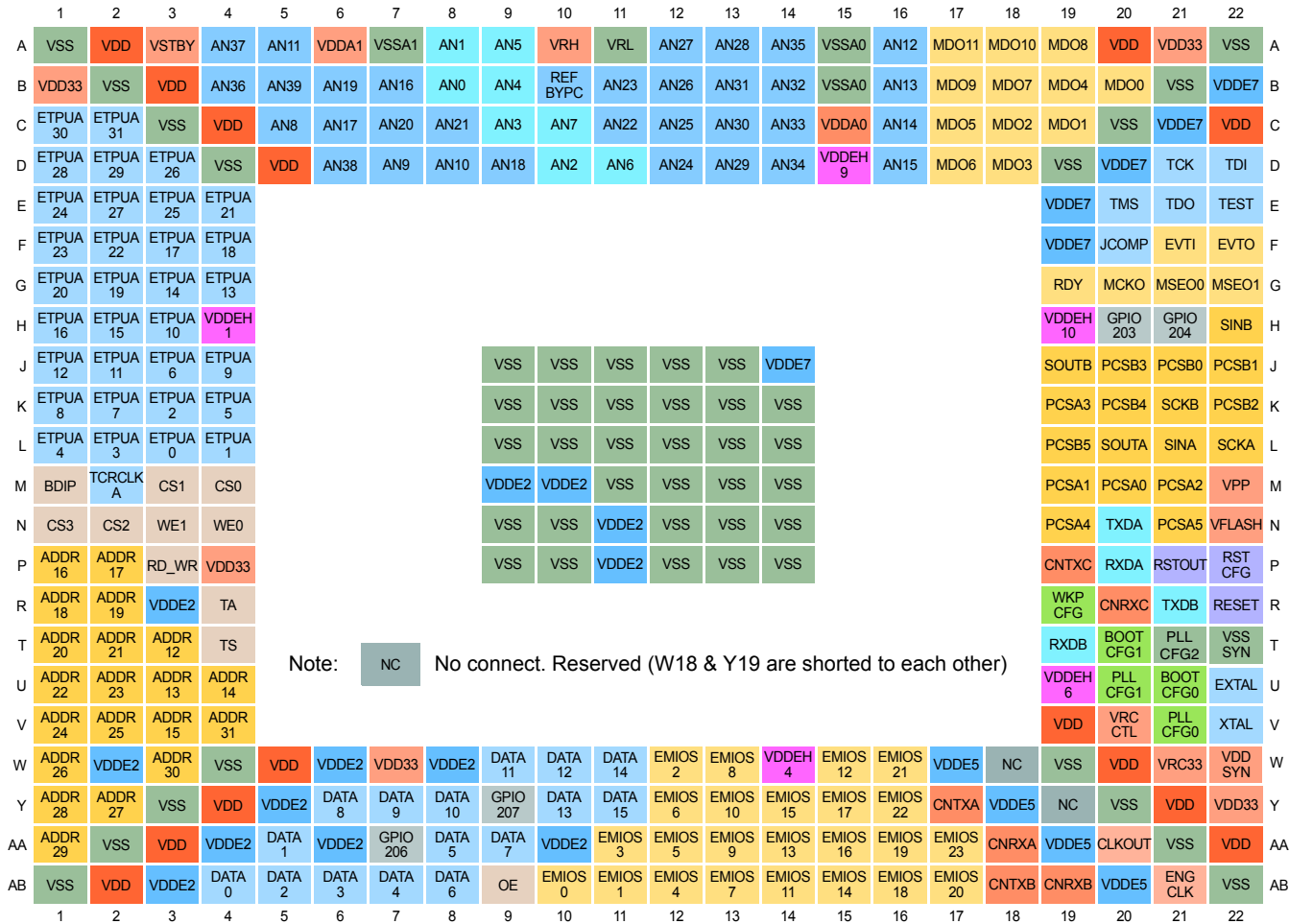
Figure 32. MPC5567 324 Package
