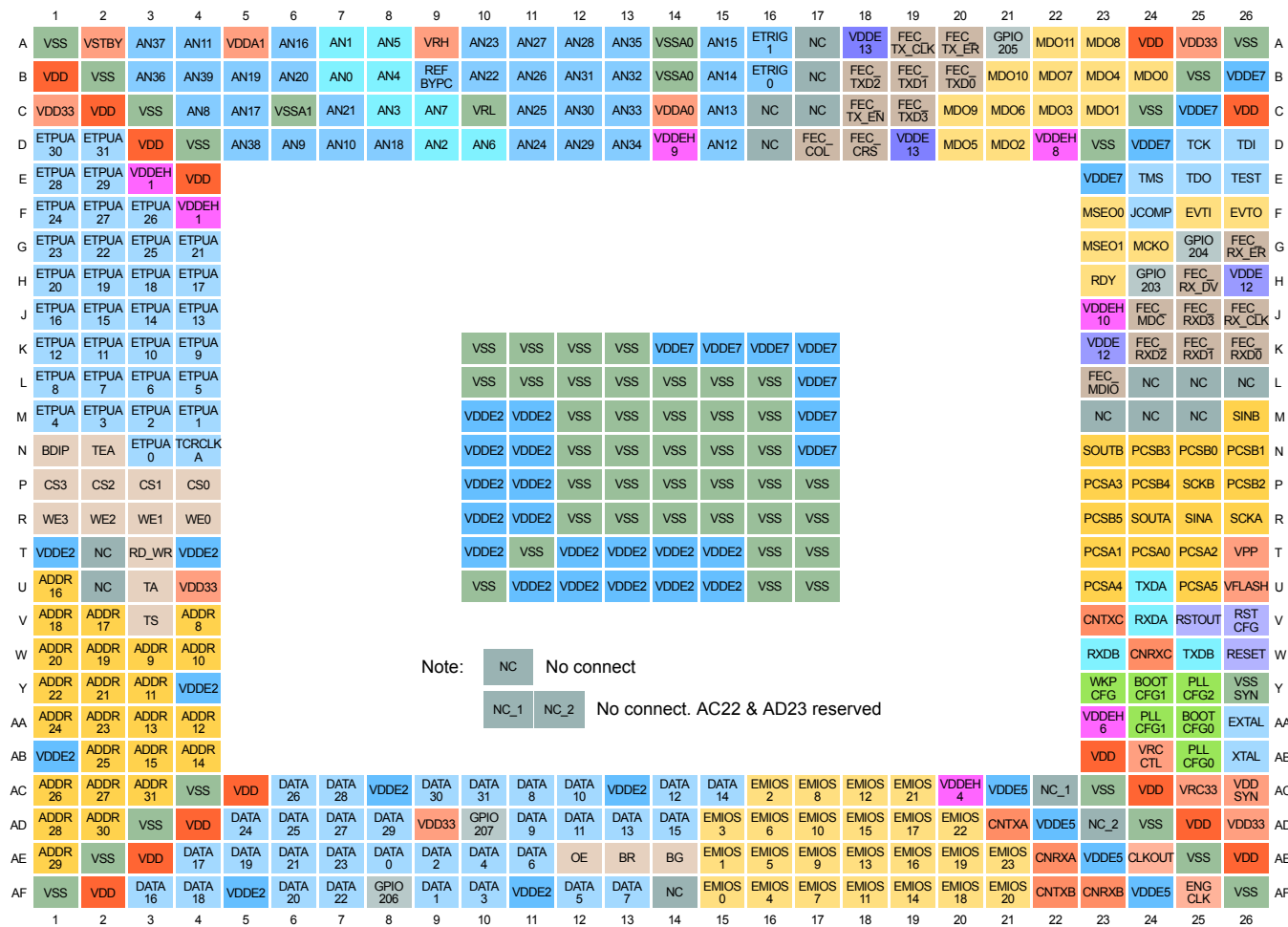
Figure 33. MPC5567 416 Package
