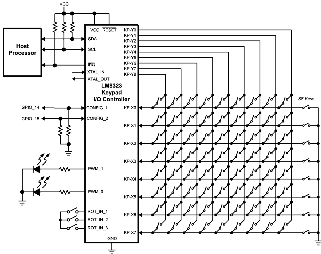
FIGURE 1. Typical Application
