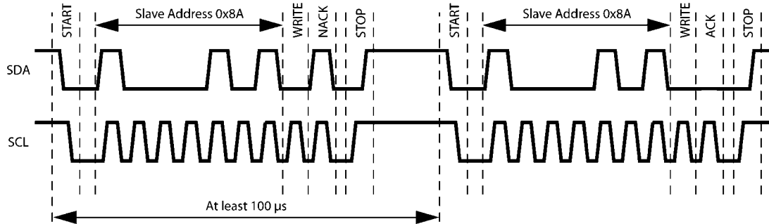
FIGURE 19. LM8323 Responds with NACK, Host Retries Command
