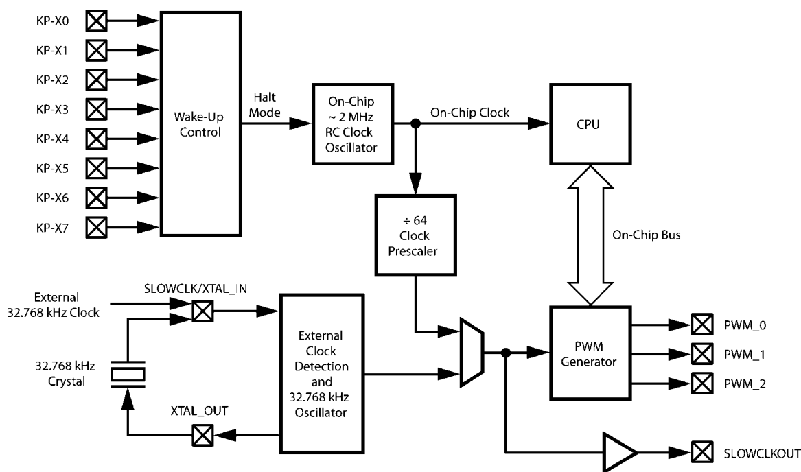
FIGURE 2. Clock Architecture
