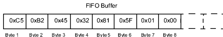
FIGURE 7. Example Event Codes Loaded in FIFO Buffer
