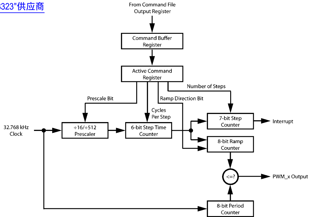
FIGURE 14. PWM Timer
