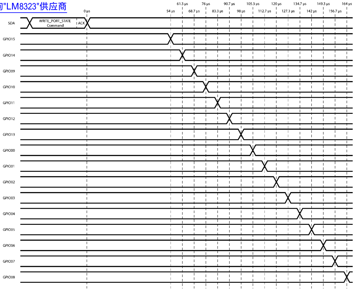
FIGURE 11. GPIO Port State Change Timing
