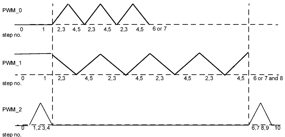
FIGURE 15. PWM Outputs
