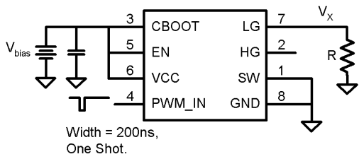
Test Circuit 3
