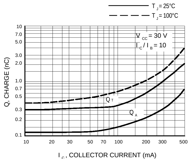
Figure 4. Charge Data
