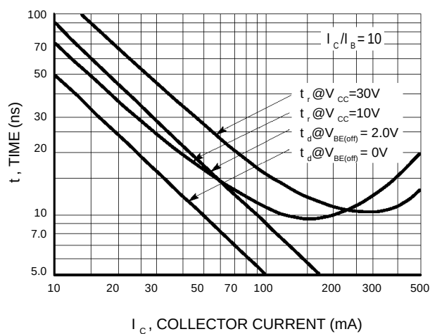
Figure 5. Turn-On Time
