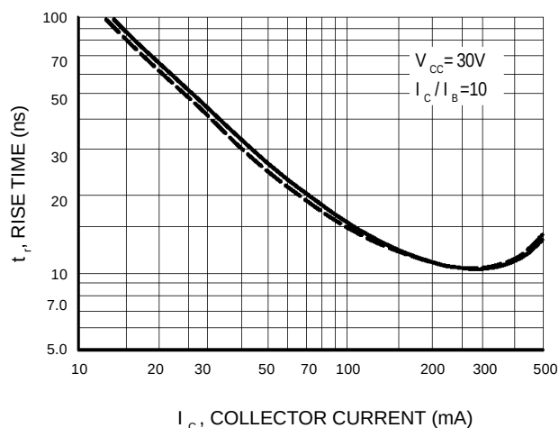
Figure 6. Rise Time
