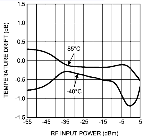
Mean Temperature Drift Error vs. RF Input Power at 300 MHz
