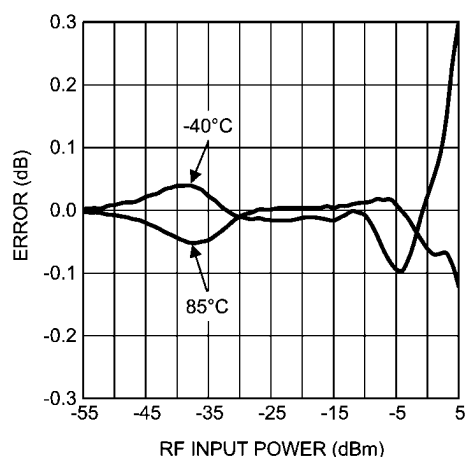
Error for 1 dB Input Power Step vs. RF Input Power at 3500 MHz
