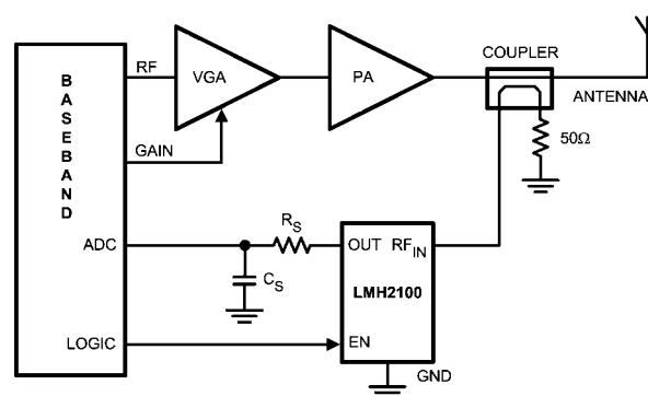
FIGURE 3. Transmit Power Control System
