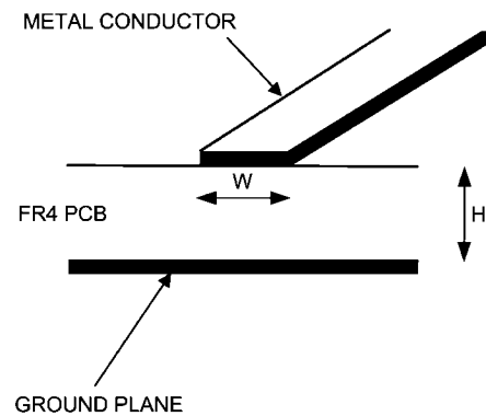
FIGURE 15. Microstrip Configuration
