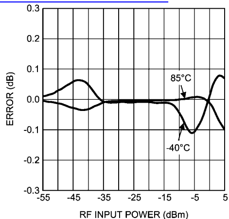
Error for 1 dB Input Power Step vs. RF Input Power at 185 MHz
