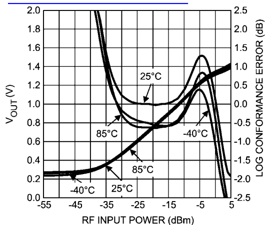
Mean Output Voltage and Log Conformance Error vs. RF Input Power at 400 MHz
