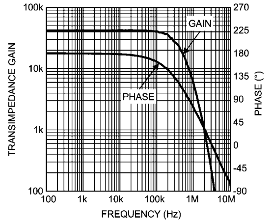
Output Amplifier Gain &amp; Phase vs. Frequency
