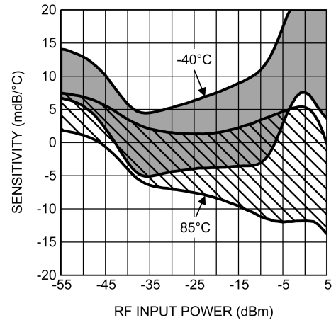
Temperature Sensitivity (Mean \pm 3 sigma) vs. RF Input Power at 1850 MHz
