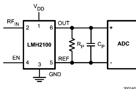
FIGURE 12. Single Ended and Differential Application
