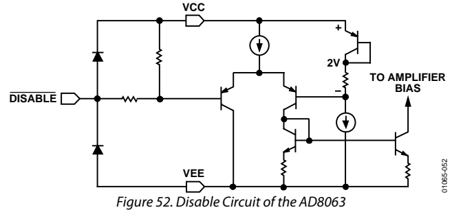
Figure 52. Disable Circuit of the AD8063
