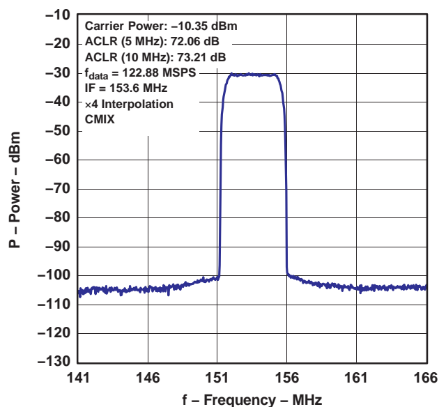
Figure 18. WCDMA TM1 : Single Carrier, PLL Off, DVDD = 1.8 V
