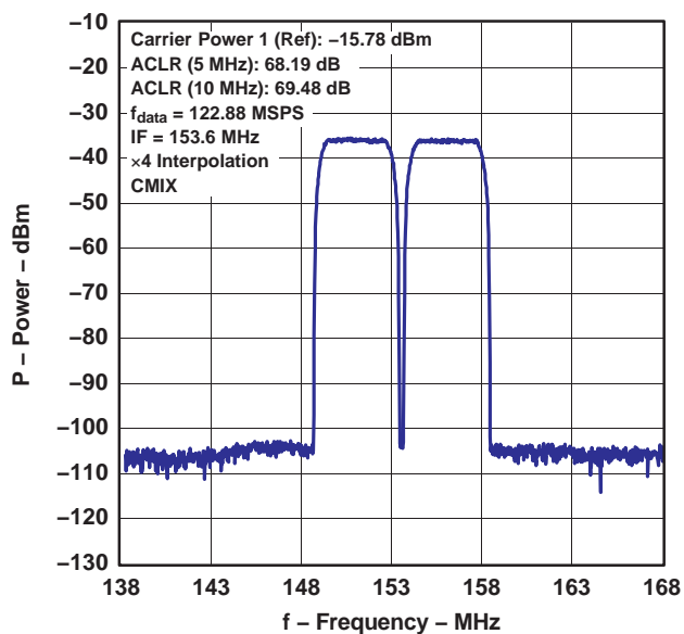
Figure 20. WCDMA TM1 : Two Carrier, PLL Off, DVDD = 1.8 V
