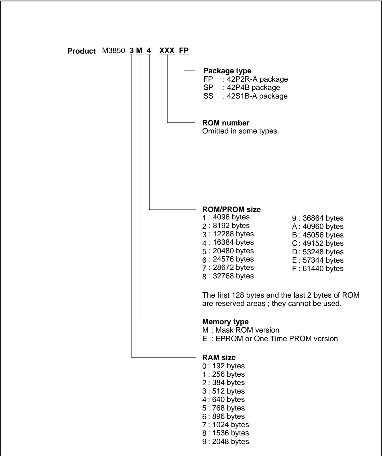
Fig. 3 Part numbering
