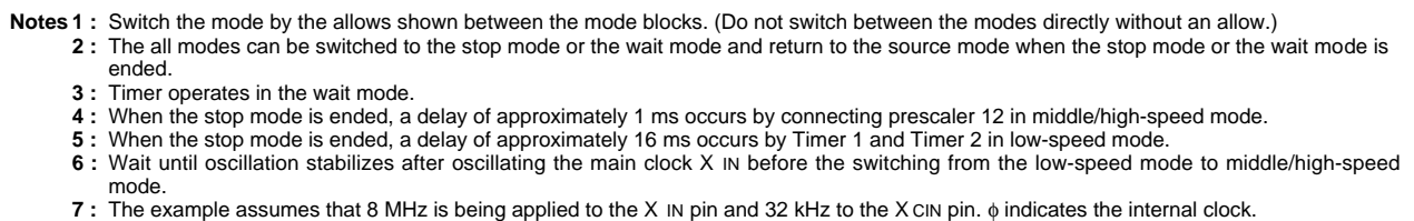
Fig. 36 State transitions of system clock
