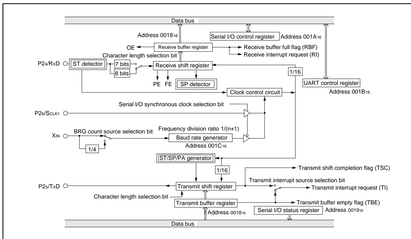
Fig.17 Block diagram of UART serial I/O
