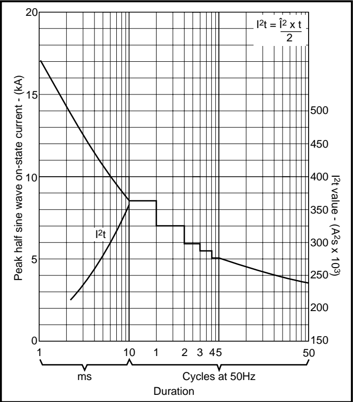
Fig. 4 Surge (non-repetitive) on-state current vs time (Thyristor or diode with 50% V_{RRM} at T_{case} = 130^{\circ}\text{C} )
