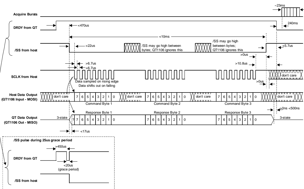
Figure 3.1 SPI Operation
