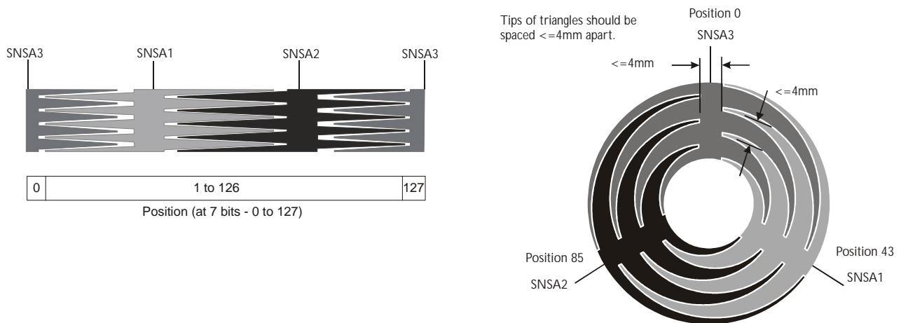
Figure 1.1 All-Metal Slider and Wheel Construction (downloadable example CAD files for wheels and sliders can be found on the Quantum website, http://www.qprox.com/toolbox/1106 )
