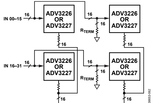
Figure 65. A 32 \times 32 Nonblocking Crosspoint Switch Array
