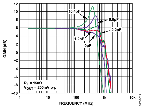
Figure 12. ADV3227 Small Signal Frequency Response, R_L = 150\Omega
