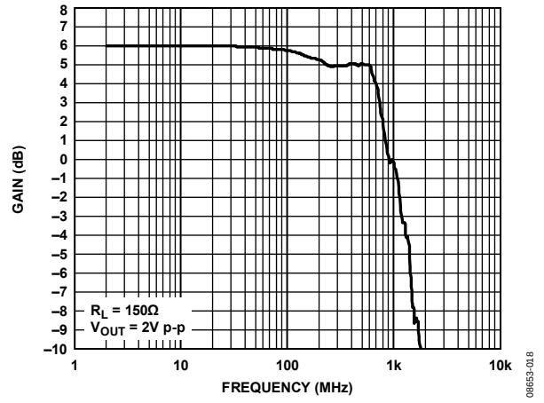
Figure 11. ADV3227 Large Signal Frequency Response
