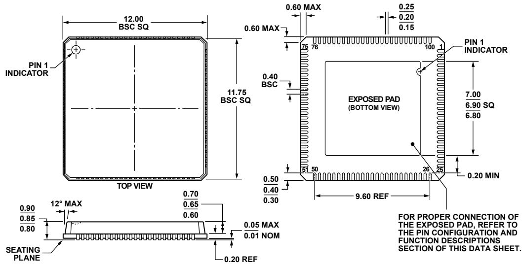
Figure 66. 100-Lead Lead Frame Chip Scale Package [LFCSP_VQ] 12 mm × 12 mm Body, Very Thin Quad (CP-100-1) Dimensions shown in millimeters
