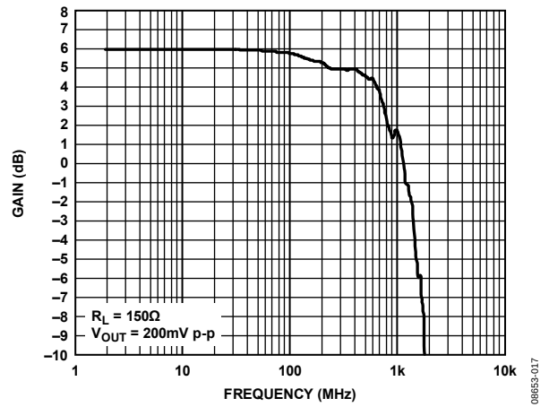
Figure 10. ADV3227 Small Signal Frequency Response
