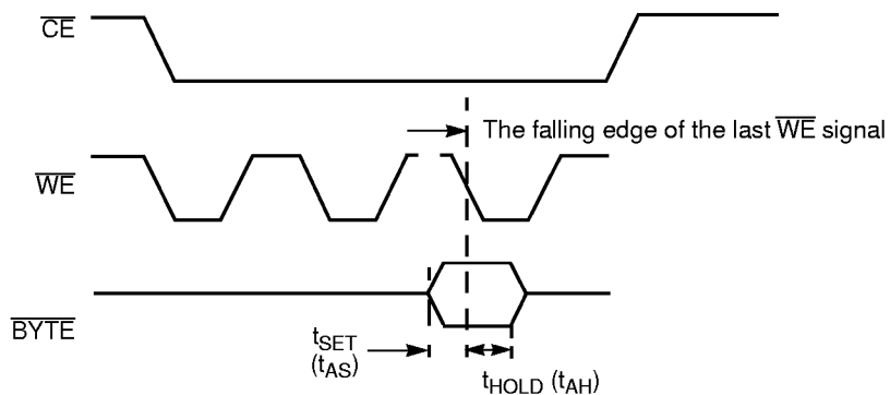
Figure 16. \overline{\text{BYTE}} Timing Diagram for Write Operations
