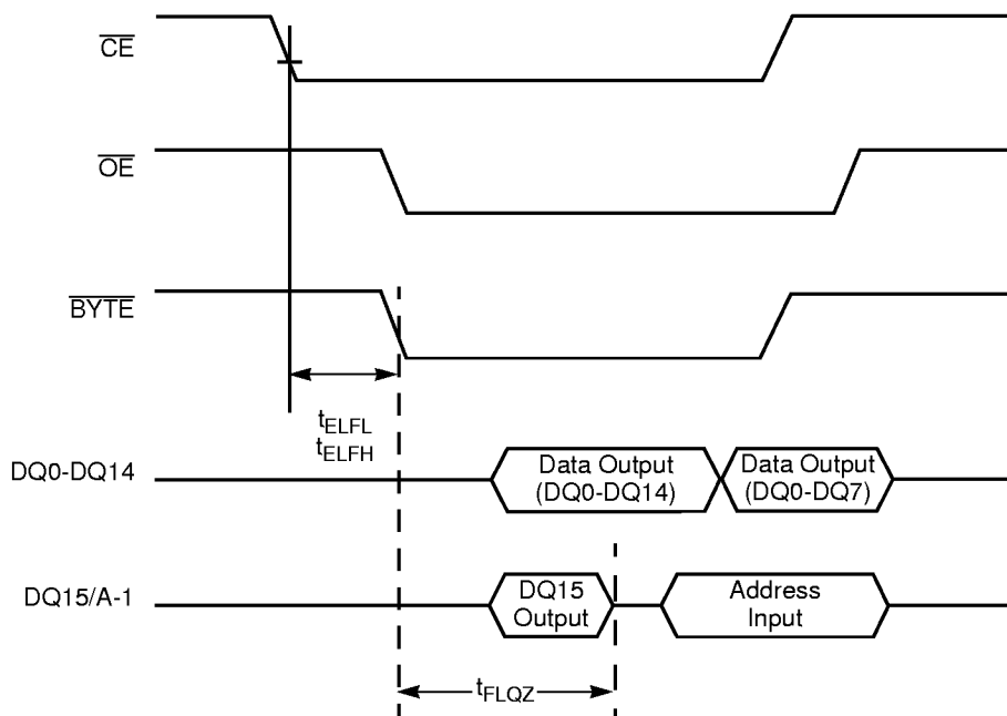
Figure 15. \overline{\text{BYTE}} Timing Diagram for Read Operation
