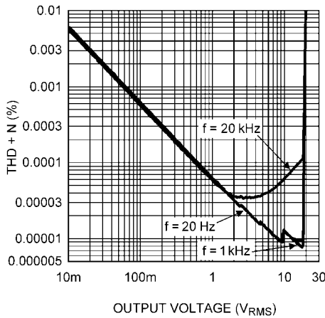
THD+N vs Output Voltage V_S = \pm 15V, R_L = 2k\Omega , Differential Input f = 20Hz, 1kHz, 20kHz, 80kHz BW
