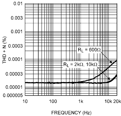
THD+N vs Frequency V_S = \pm 15V, V_O = 2V_{RMS} , Single-ended Input R_L = 600\Omega, 2k\Omega, 10k\Omega, 80kHz BW
