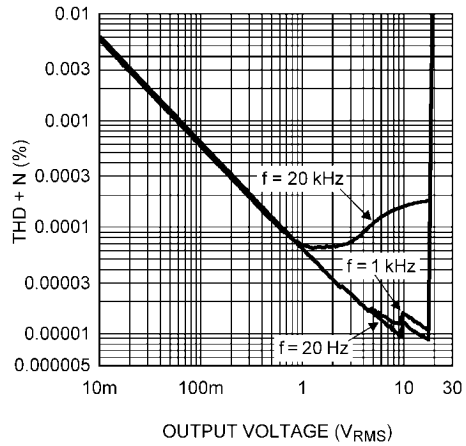
THD+N vs Output Voltage V_S = \pm 15V, R_L = 600\Omega , Differential Input f = 20Hz, 1kHz, 20kHz, 80kHz BW
