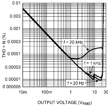
THD+N vs Output Voltage V_S = \pm 18V, R_L = 600\Omega , Differential Input f = 20Hz, 1kHz, 20kHz, 80kHz BW
