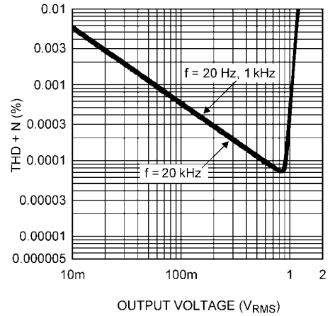
THD+N vs Output Voltage V_S = \pm 2.5V, R_L = 2k\Omega , Differential Input f = 20Hz, 1kHz, 20kHz, 80kHz BW
