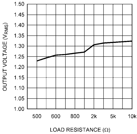
Output Voltage vs Load Resistance V_S = \pm 12.5V , R_L = 500\Omega - 10k\Omega THD+N \leq 1\% , 80kHz BW
