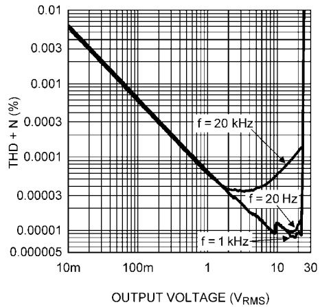
THD+N vs Output Voltage V_S = \pm 18V, R_L = 2k\Omega , Differential Input f = 20Hz, 1kHz, 20kHz, 80kHz BW
