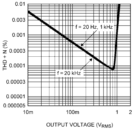
THD+N vs Output Voltage V_S = \pm 15V, R_L = 600\Omega , Differential Input f = 20Hz, 1kHz, 20kHz, 80kHz BW
