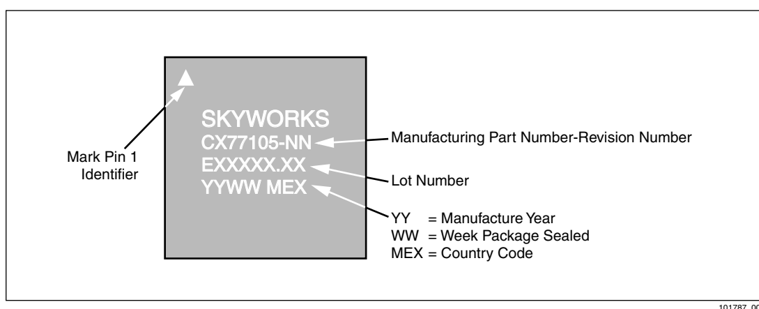
Figure 13. Typical Case Markings
