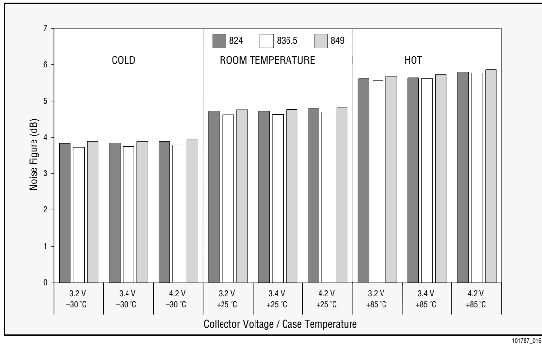
Figure 8. Noise Figure as Function of Operating Conditions
