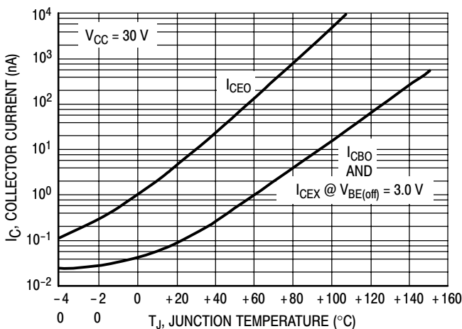
Figure 20. Typical Collector Leakage Current
