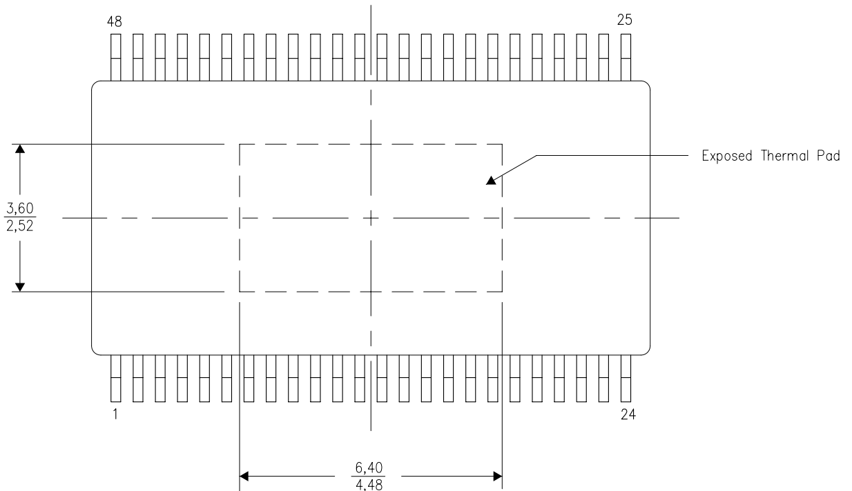
Top View
