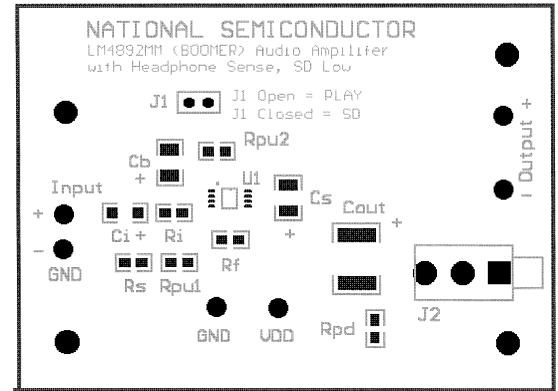
Silk Screen
