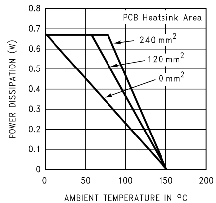
Power Derating Curves vs for 8 Bump microSMD
