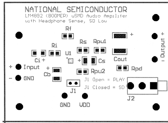
Silk Screen
