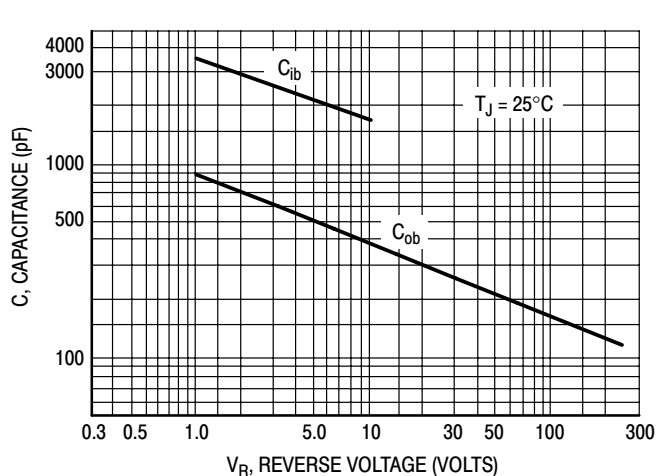
Figure 2. Capacitances
