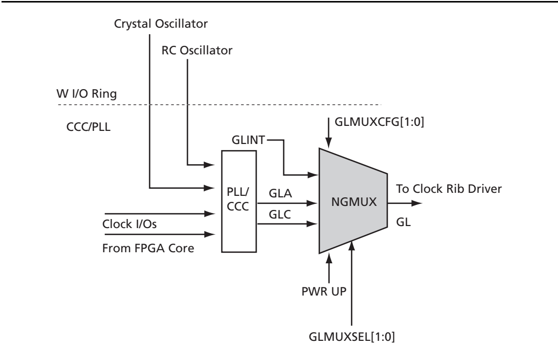
Figure 2-24 • NGMUX
