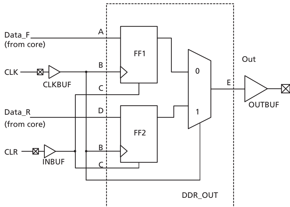
Figure 2-94 • DDR Output Support in Fusion Devices
