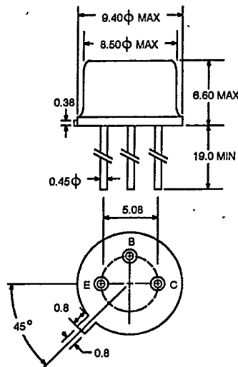
OUTLINE 14 (TO-39)
