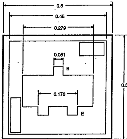
NE74000 (CHIP)
