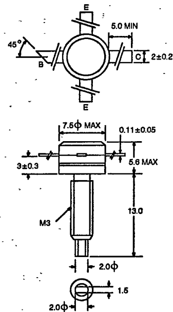
OUTLINE 20
