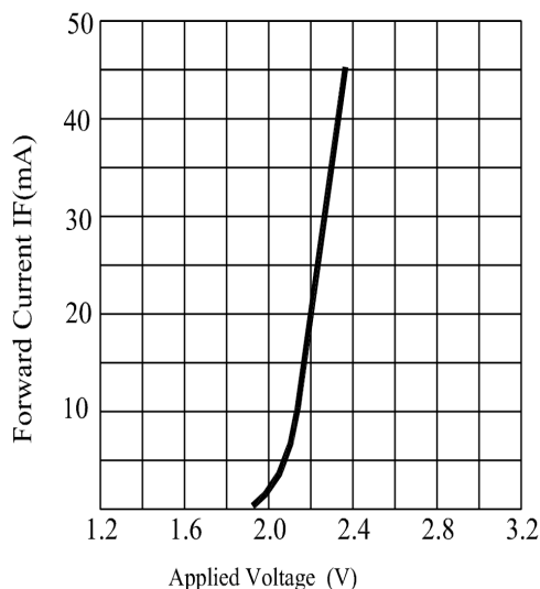
FORWARD CURRENT VS. APPLIED VOLTAGE
