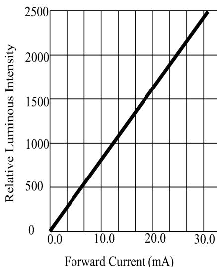
FORWARD CURRENT VS. LUMINOUS INTENSITY
