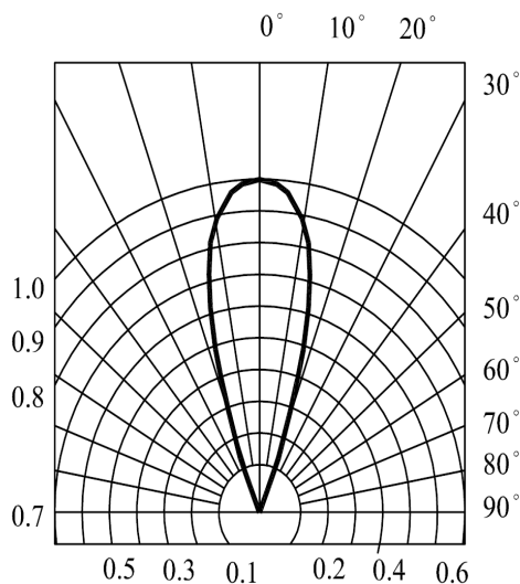
RADIATION DIAGRAM
