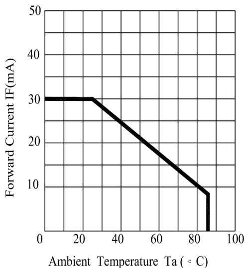
AMBIENT TEMPERATURE VS. FORWARD CURRENT
