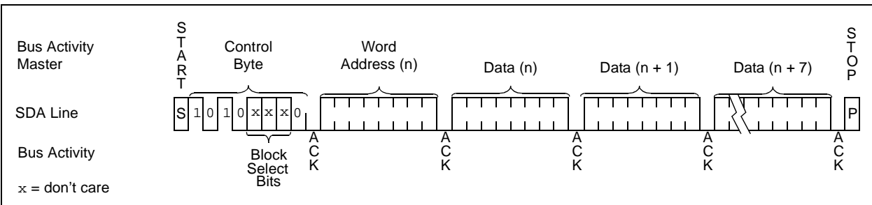
FIGURE 5-2: PAGE WRITE
