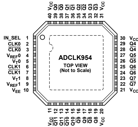
Figure 2. Pin Configuration
