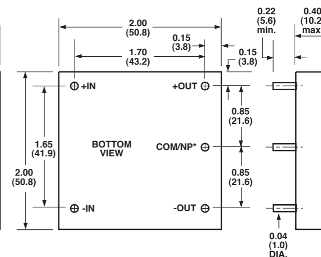
ALTERNATE PIN CONFIGURATION SUFFIX "S"
