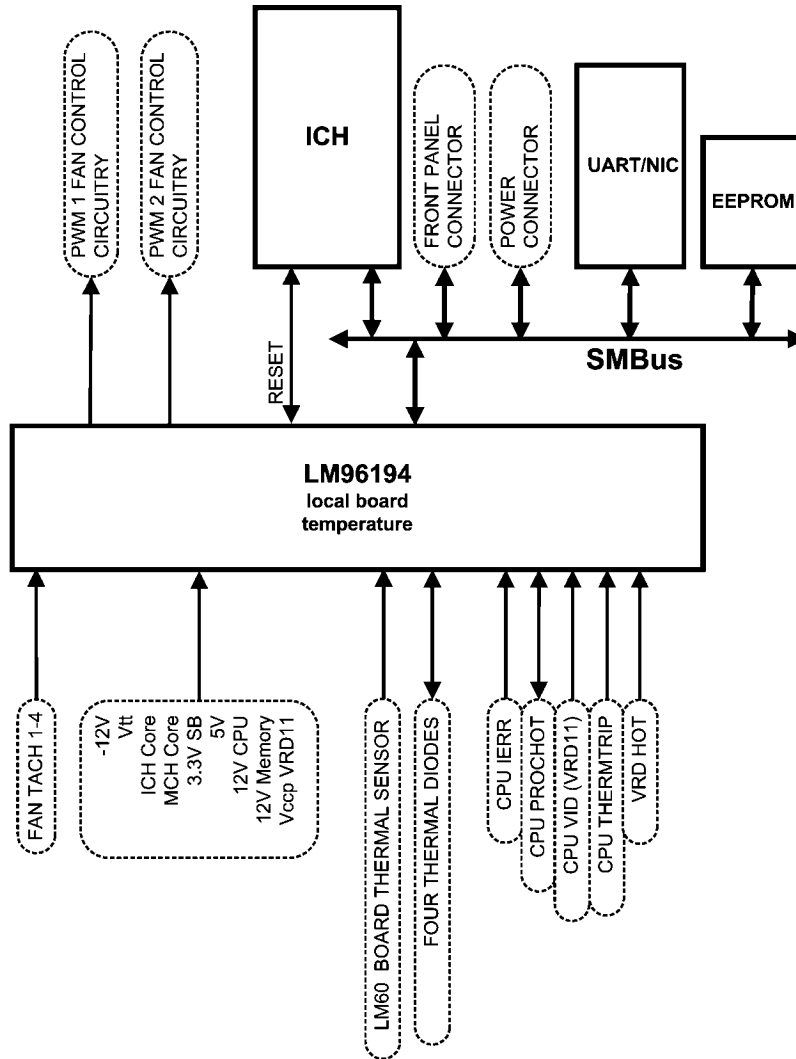
FIGURE 1. Workstation Management
