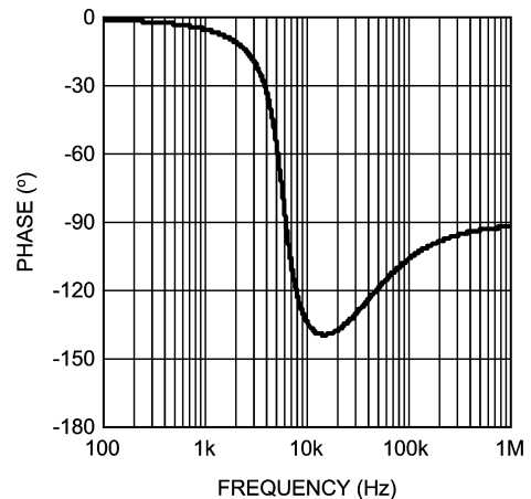
FIGURE 9. Power Stage Gain and Phase
