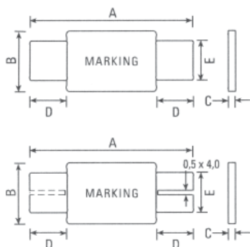
Dimensions (mm)
