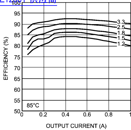
查询"LMZ12001"供应商 Efficiency 6V Input @ 85°C
