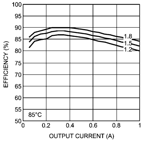
Efficiency 4.5V Input @ 85°C
