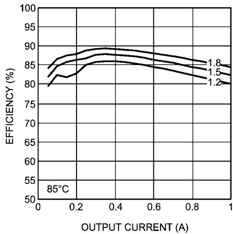
Efficiency 5V Input @ 85°C
