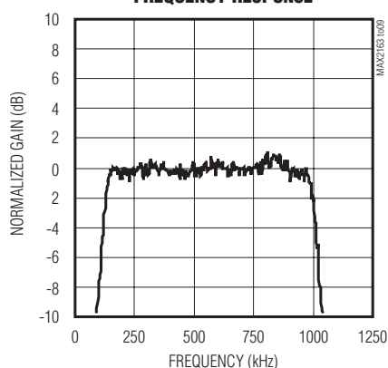
1-SEGMENT BASEBAND FILTER FREQUENCY RESPONSE
