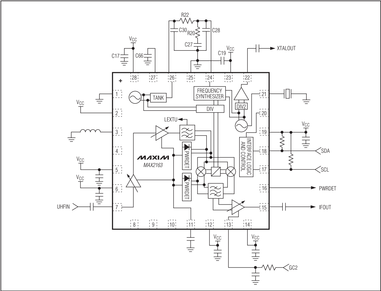
Typical Application Circuit
