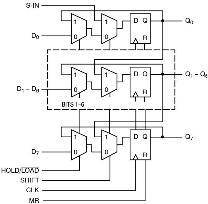
Figure 2. Logic Diagram
