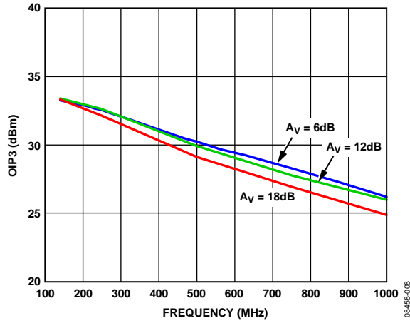
Figure 11. OIP3 vs. Frequency at A_V = 6\text{ dB} , A_V = 12\text{ dB} , and A_V = 18\text{ dB} , V_{OUT} = 0.45\text{ V p-p/Tone} , 2 MHz Spacing
