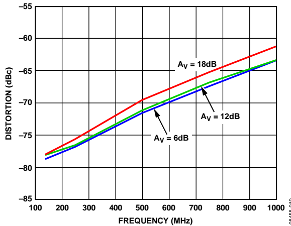
Figure 13. Two Tone IMD3 vs. Frequency, A_V = 6\text{ dB} , A_V = 12\text{ dB} , and A_V = 18\text{ dB} , V_{OUT} = 0.9\text{ V p-p/Tone} , 2 MHz Spacing
