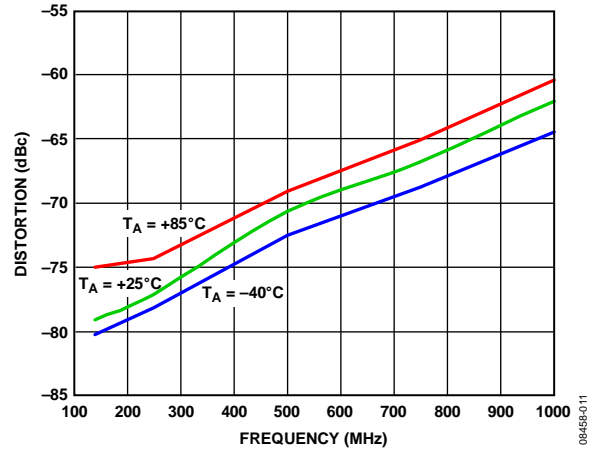
Figure 14. Two Tone IMD3 vs. Frequency at T_A = -40^\circ\text{C} , T_A = +25^\circ\text{C} , and T_A = +85^\circ\text{C} , A_V = 6\text{ dB} , V_{OUT} = 0.45\text{ V p-p/Tone} , 2 MHz Spacing
