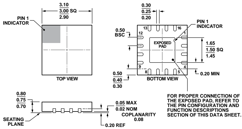
Figure 46. 16-Lead Lead Frame Chip Scale Package [LFCSWQ] 3 mm × 3 mm Body, Very Very Thin Quad (CP-16-27) Dimensions shown in millimeters
