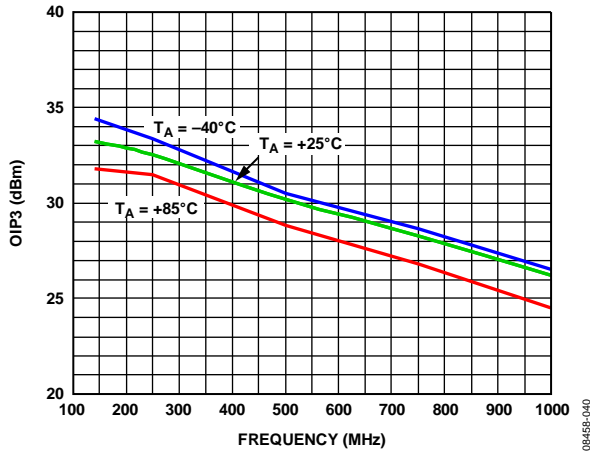
Figure 12. OIP3 vs. Frequency at A_V = 6\text{ dB} , T_A = -40^\circ\text{C} , T_A = +25^\circ\text{C} , and T_A = +85^\circ\text{C} , V_{OUT} = 0.45\text{ V p-p/Tone} , 2 MHz Spacing
