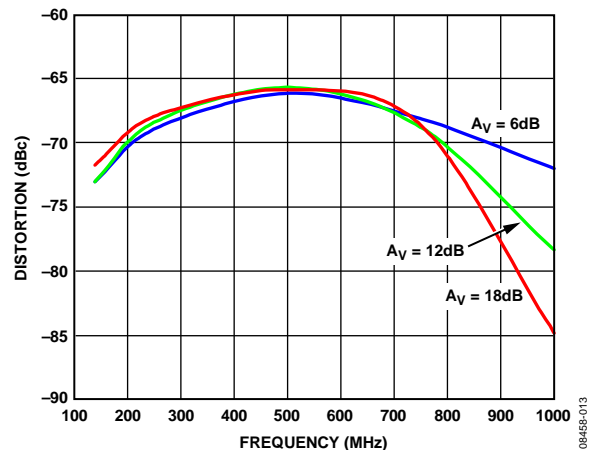
Figure 16. HD3 vs. Frequency at A_V = 6\text{ dB} , A_V = 12\text{ dB} , and A_V = 18\text{ dB} , V_{OUT} = 0.9\text{ V p-p}
