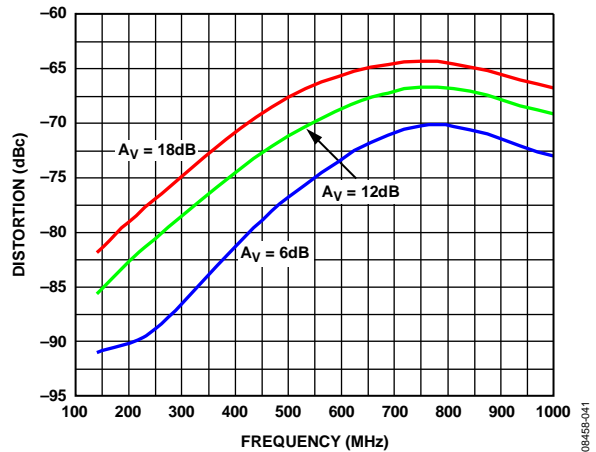
Figure 15. HD2 vs. Frequency at A_V = 6\text{ dB} , A_V = 12\text{ dB} , and A_V = 18\text{ dB} , V_{OUT} = 0.9\text{ V p-p}
