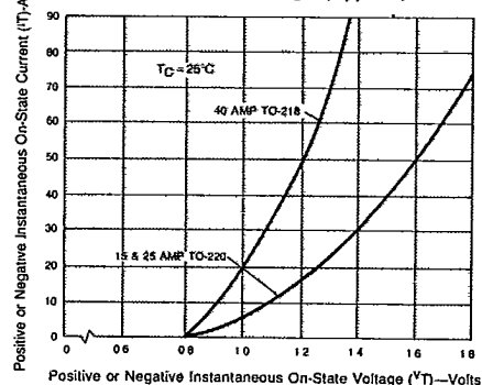
FIGURE 3 — On-State Current vs On-State Voltage (Typical)
