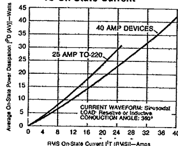
FIGURE 9B — Power Dissipation (Typ.) vs On-State Current
