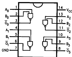
Pin Assignment for DIP, SSOP, TSSOP and SOIC
