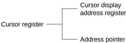
Figure 34. Cursor addressing
