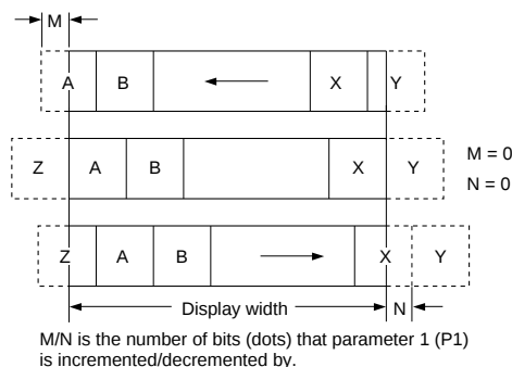
Figure 21. Horizontal scrolling
