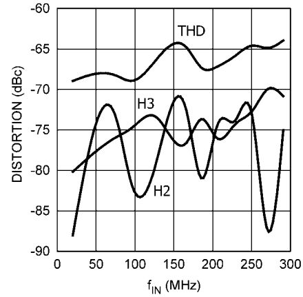
Distortion vs. f_{IN} ( f_{CLK} = 52\text{MSPS} , A_{IN} = -9\text{dBFS} )
