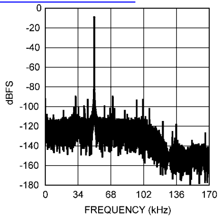
查询"LM97593"供应商 Spectral Response @ 250MHz Input ( f_{\text{CLK}} = 65\text{MSPS} , A_{\text{IN}} = -9\text{dBFS} )
