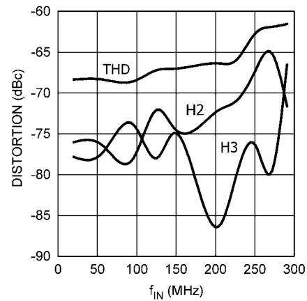
Distortion vs. f_{IN} ( f_{CLK} = 65\text{MSPS} , A_{IN} = -9\text{dBFS} )
