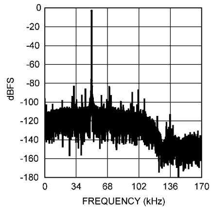
Spectral Response @ 250MHz Input ( f_{\text{CLK}} = 65\text{MSPS} , A_{\text{IN}} = -3\text{dBFS} )
