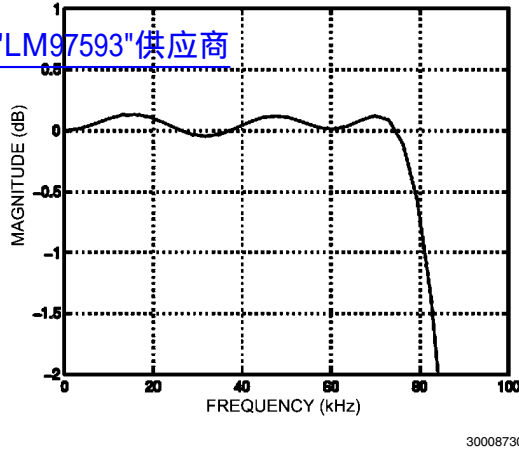
FIGURE 32. CIC, F1, &amp; F2 GSM Passband Flatness
