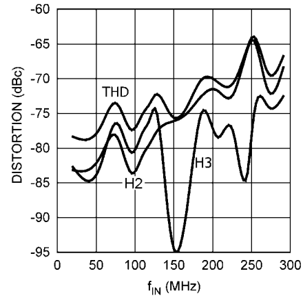
Distortion vs. f_{IN} ( f_{CLK} = 52\text{MSPS} , A_{IN} = -3\text{dBFS} )
