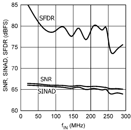
SNR, SINAD, SFDR vs. f_{IN} ( f_{CLK} = 65\text{MSPS} , A_{IN} = -9\text{dBFS} )
