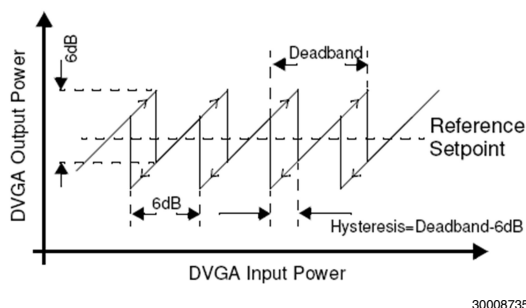
FIGURE 37. AGC Setup
