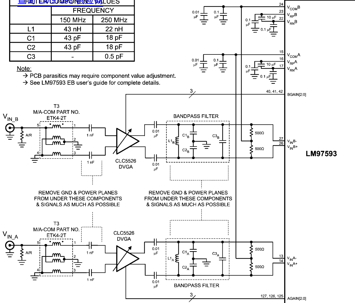
FIGURE 45. Application Circuit
