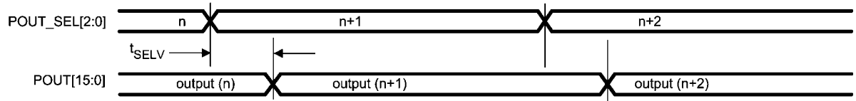
FIGURE 10. LM97593 Parallel Output Select Timing
