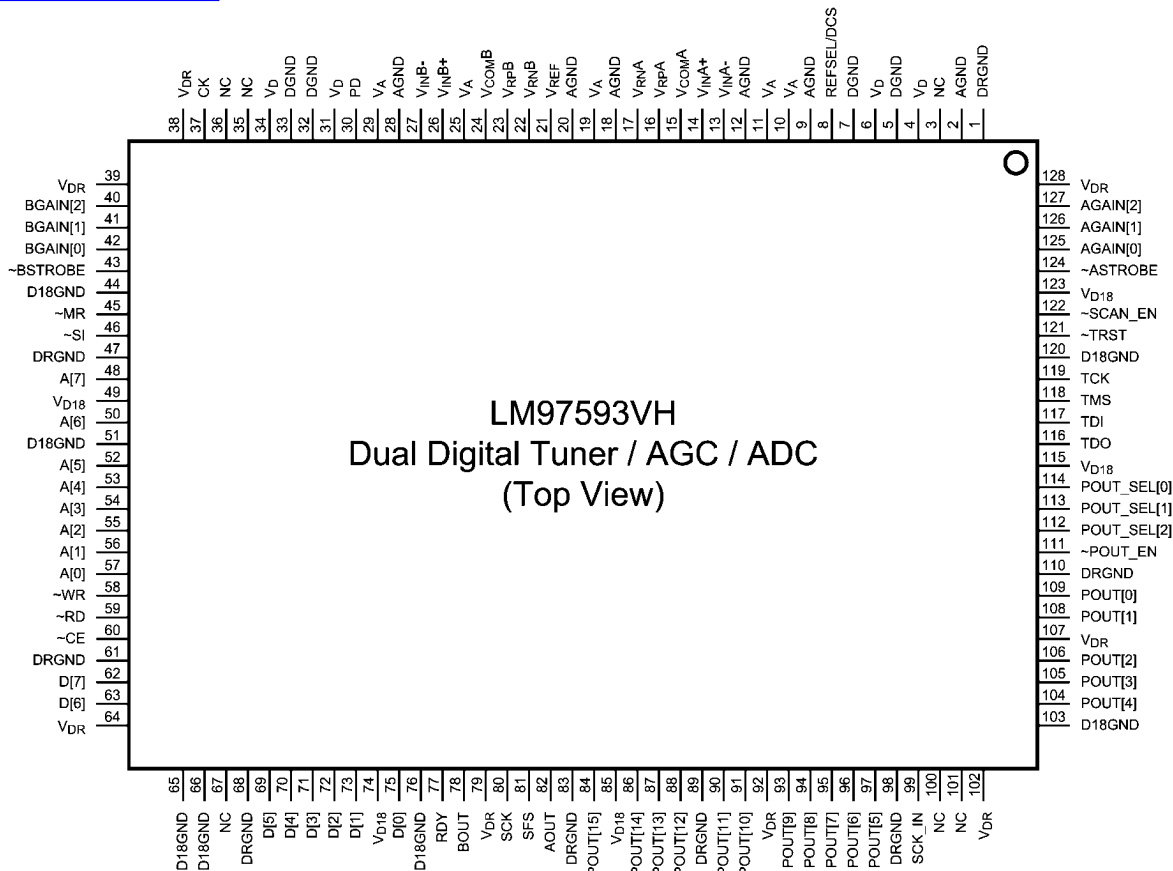
FIGURE 2. LM97593VH PQFP Pinout
