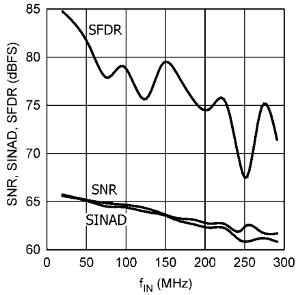
SNR, SINAD, SFDR vs. f_{IN} ( f_{CLK} = 52\text{MSPS} , A_{IN} = -3\text{dBFS} )
