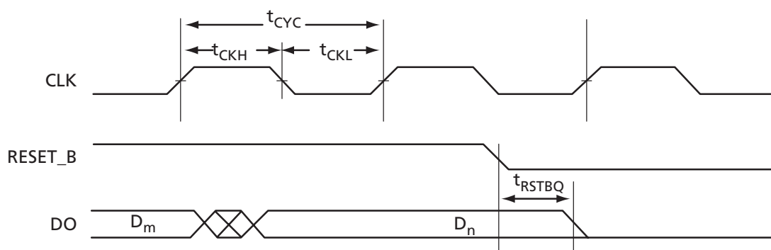
Figure 2-57 • RAM Reset
