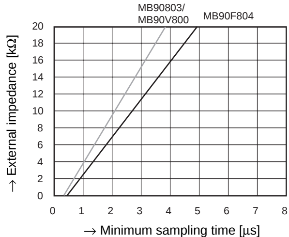
The relationship between external impedance and minimum sampling time
