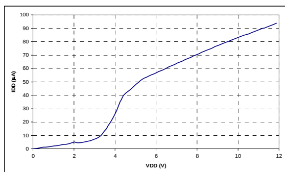
Figure 4: I DD Quiescent (I DD_QST ) vs. V DD
