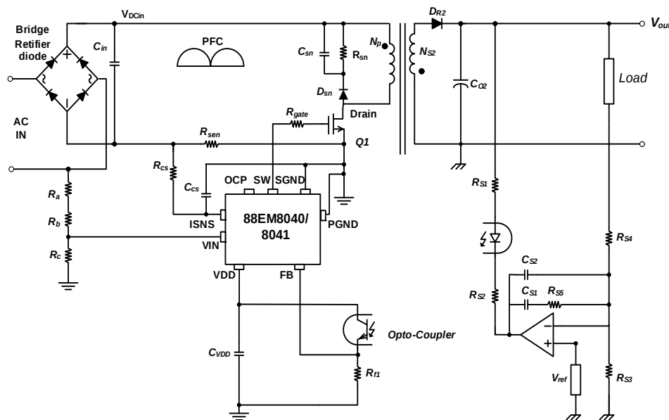
Figure 1: PFC Flyback Circuit Diagram
