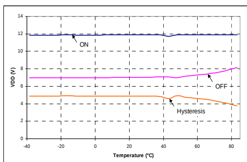
Figure 7: V_{DD} On/Off vs. Temperature
