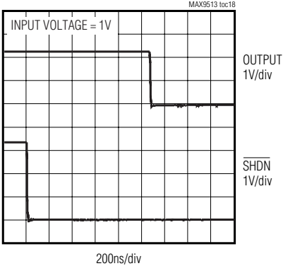
DISABLE TIME
