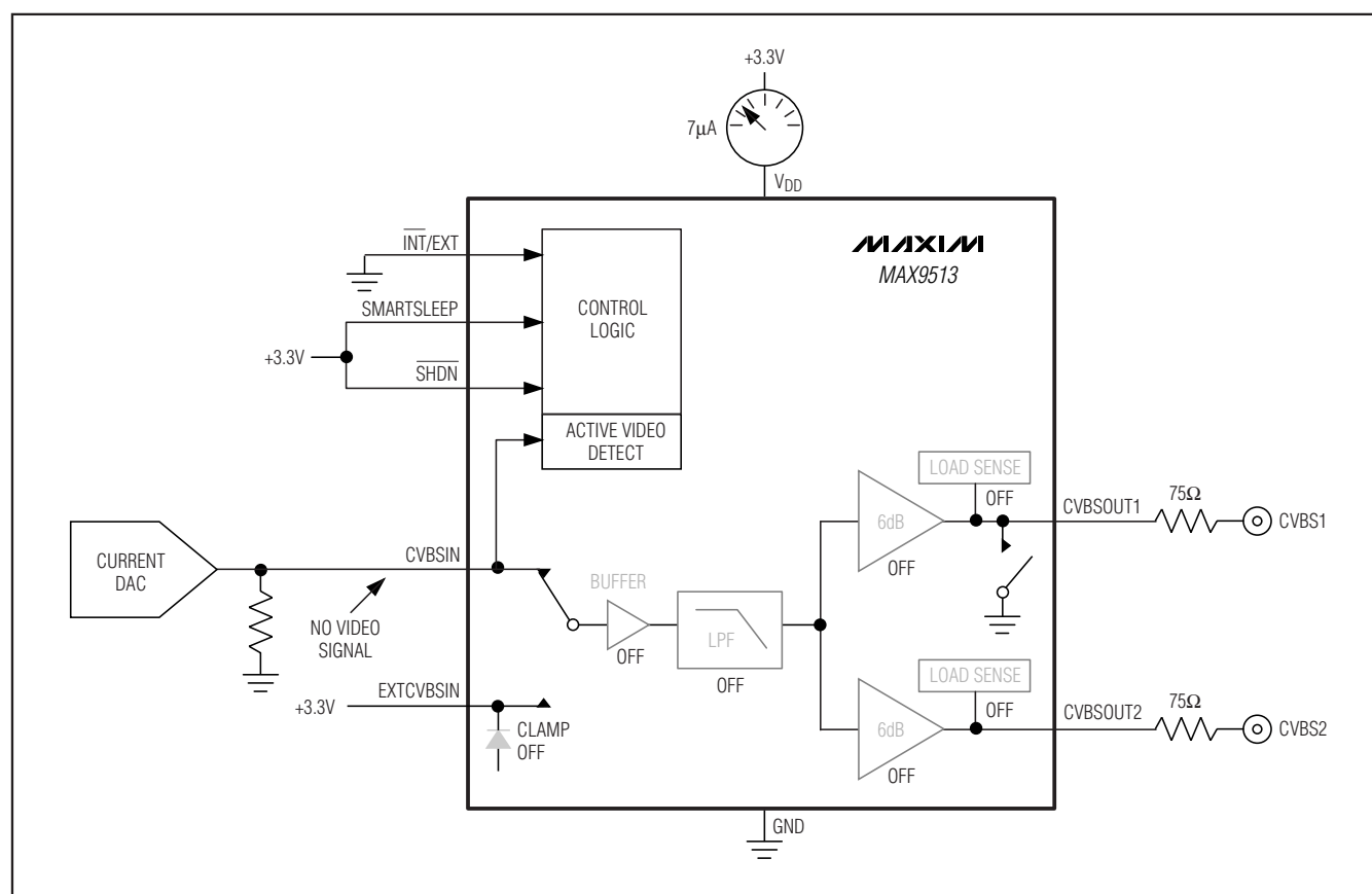
Figure 2. Standby Mode
