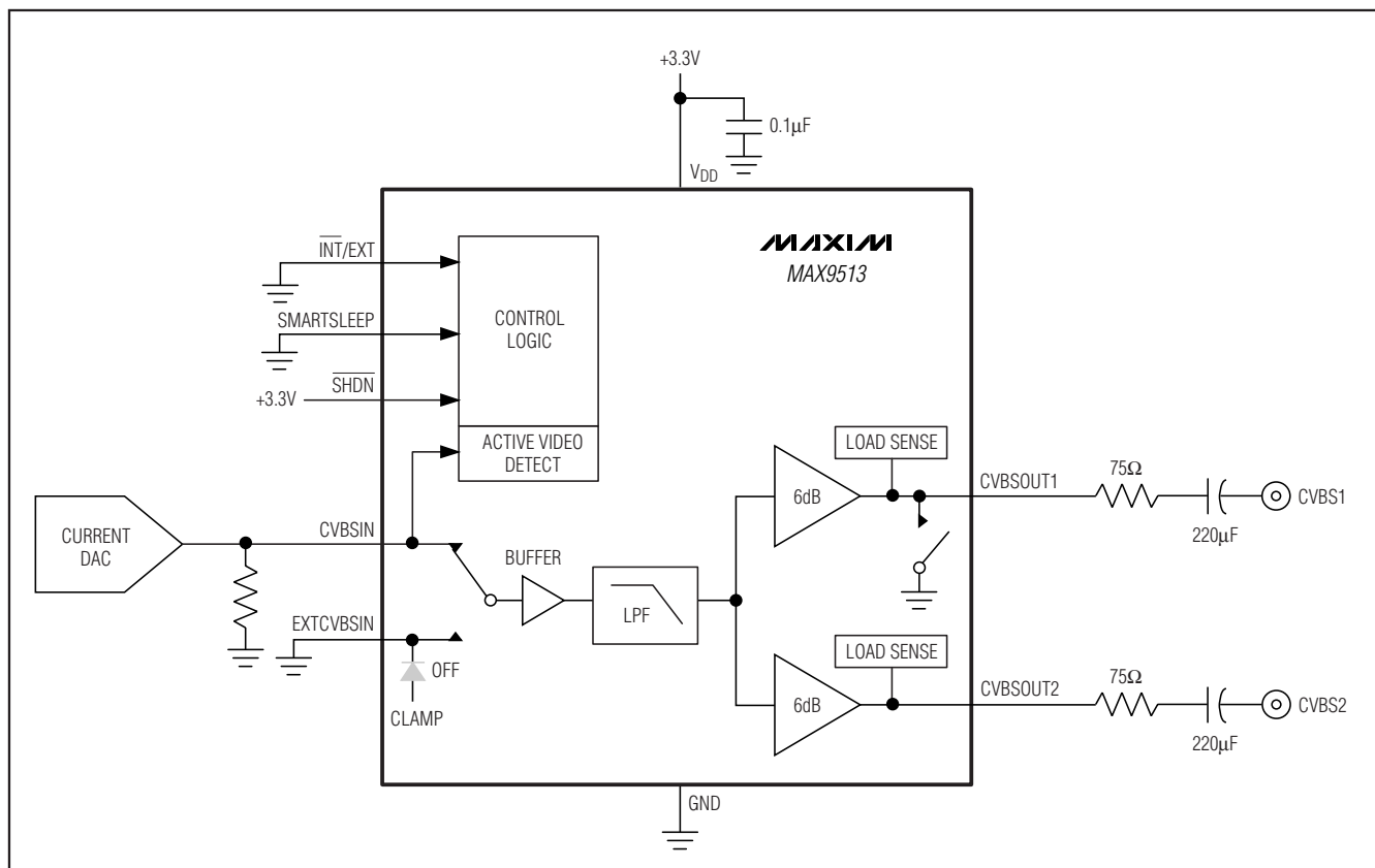
Figure 9. AC-Coupled Outputs
