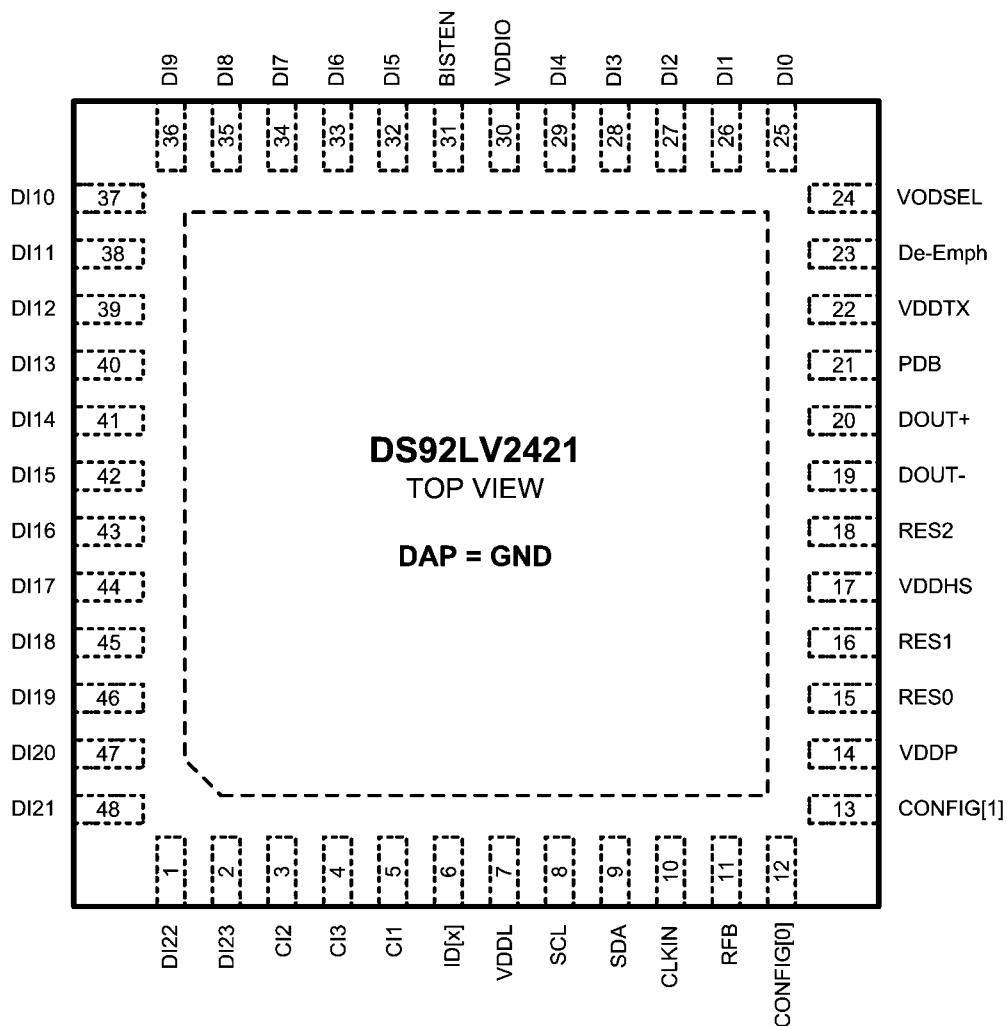
Serializer - DS92LV2421 — Top View
