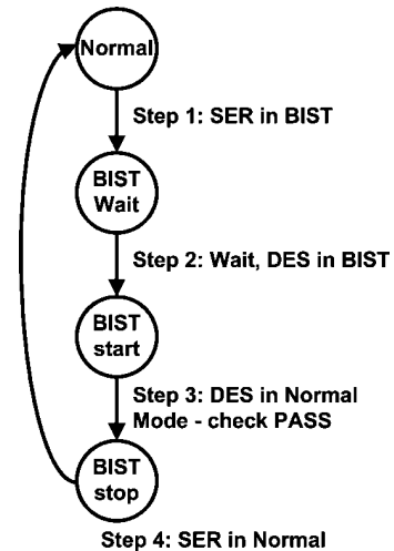
FIGURE 26. BIST Mode Flow Diagram
