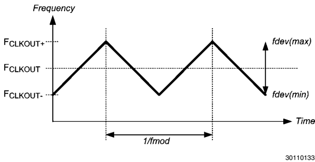
FIGURE 20. SSCG Waveform
