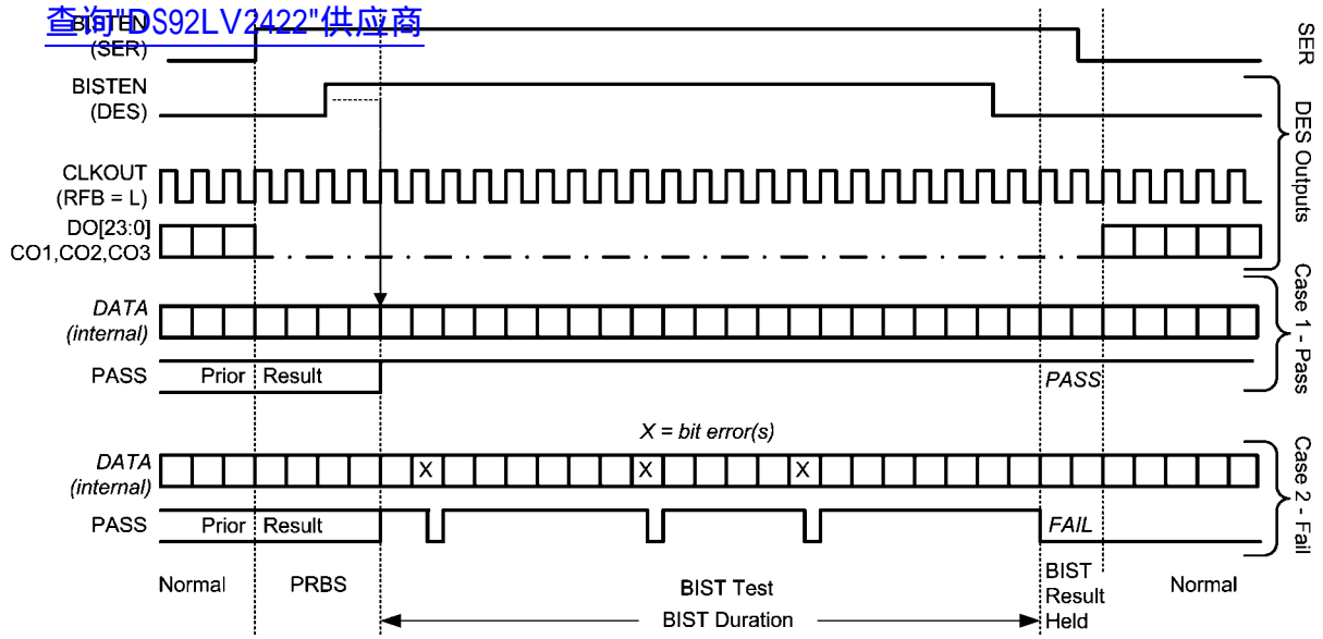
FIGURE 27. BIST Waveforms
