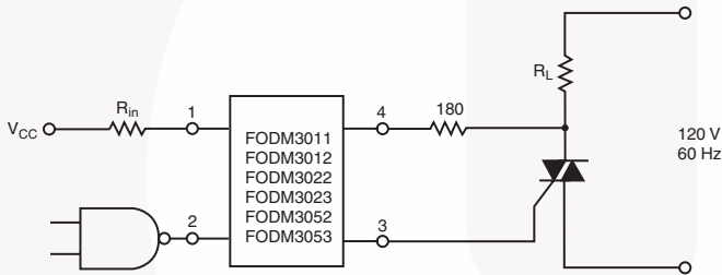
Figure 9. Resistive Load
